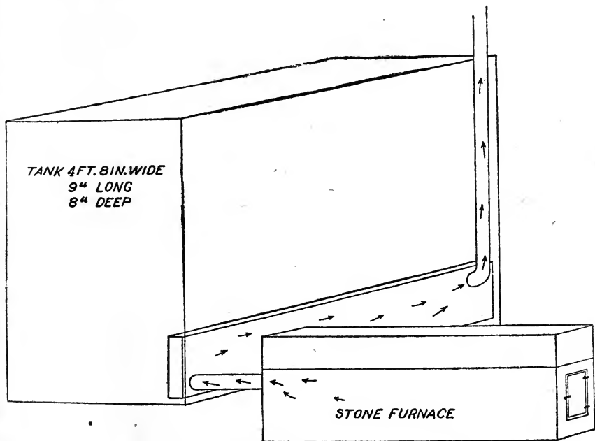
FIG. 5.—Tank with heating appliance.
