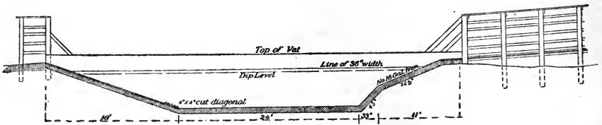
FIG. 7.—Vertical section of dipping vat with slide chute.
