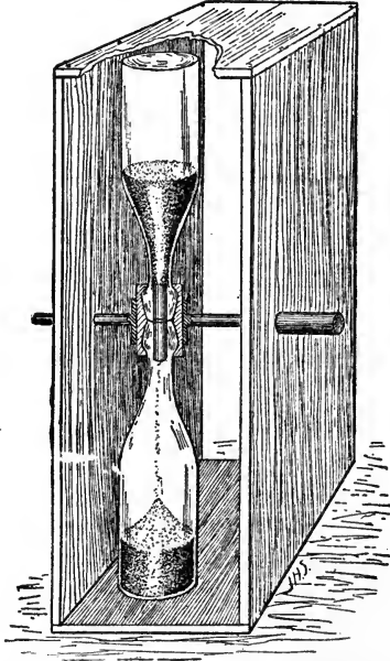
FIG. 4.—Sand glass. For timing the animals in the dip. Is made of two ordinary ketchup bottles connected by a hollow wooden cork, placed in a box, and the box hung on a pin through the center to revolve, as shown in the illustration.
