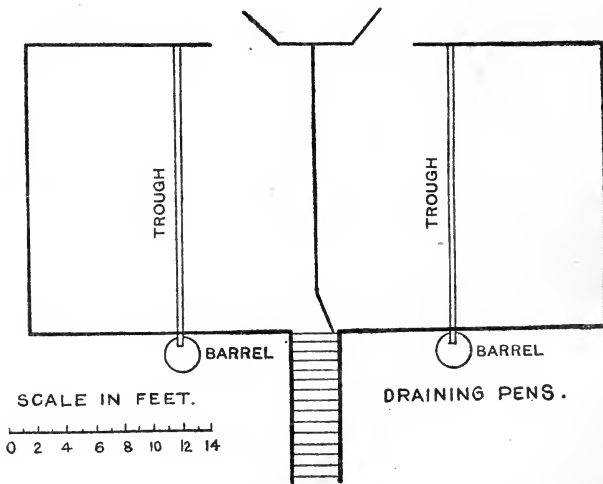
FIG. 15.—Draining pens.
