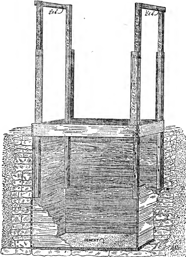
FIG. 2.—Vat. Tank 10 ft. deep, 4 ft. wide, 9 ft. in ground. Should contain from 5½ to 6 ft. of dip. Standards 4 by 4 in. by 16 ft. long, bolted to tank inside, to extend 6 ft. inside of tank, to act as guides to cage; 2 by 6 in. plank 6 ft. long nailed to outside of standards; 2 by 4 or 2 by 6 in. braces across top of standards. The tank should be built of 2-in. plank and joined with a tongue, the ends of the tank mortised in, the joints coated with lead. The braces are 4 by 4 in. The tank, being placed in the ground and packed solid, does not require much bracing. The tank should be laid in cement bottom, with stone and mortar about sides.
