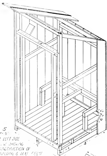
2- SIDE VIEW
