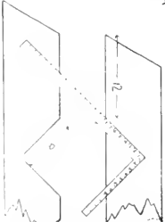
9- METHOD OF MARKING OUT SIDE WINDOWS.
