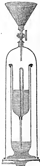
SYPHON IN VACUO.
