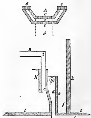
Fireplace.
