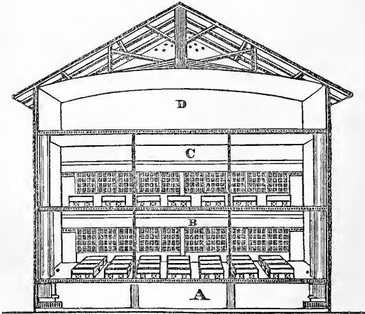
Fig. 2. Transverse Section.
