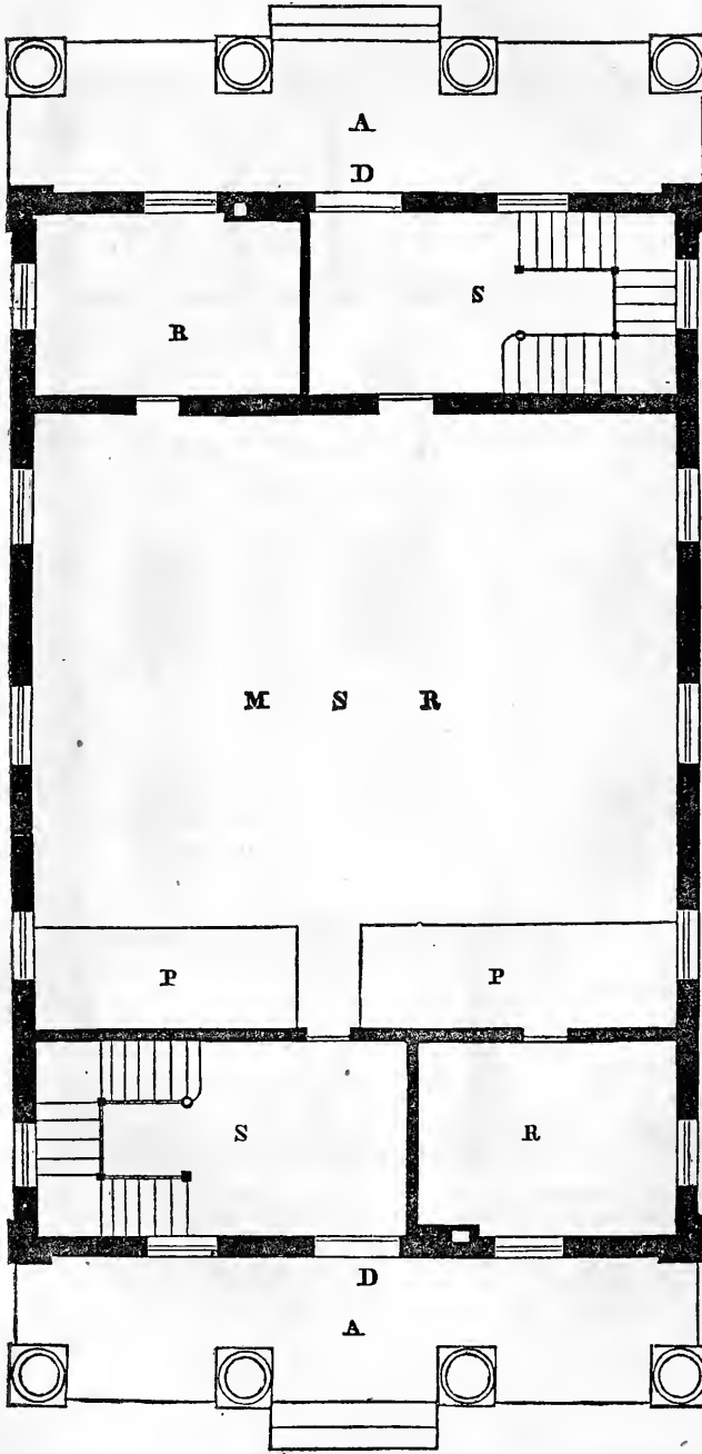
Fig. 5.—LOWER STORY.
