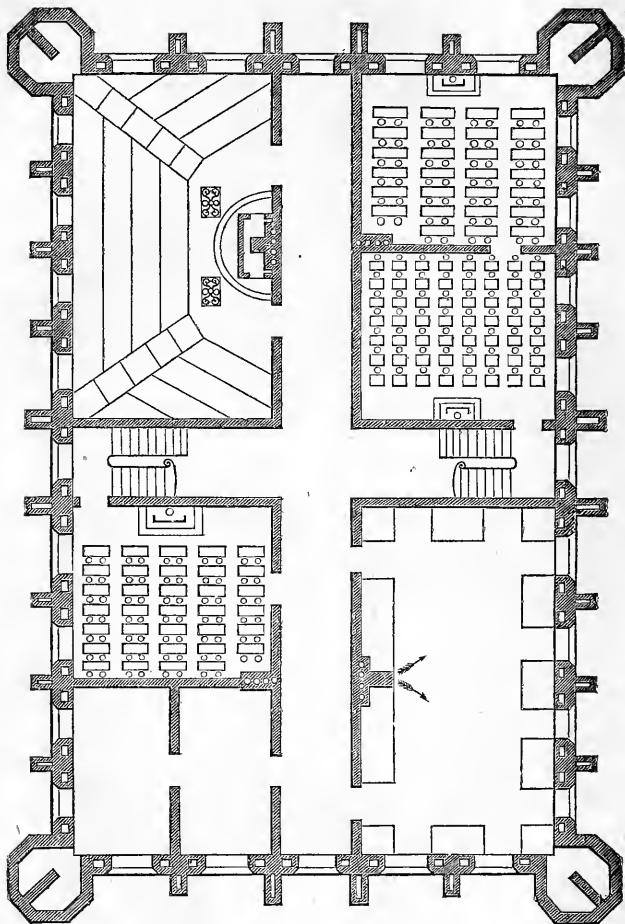
FIG 5.—PLAN OF FIRST STORY.
