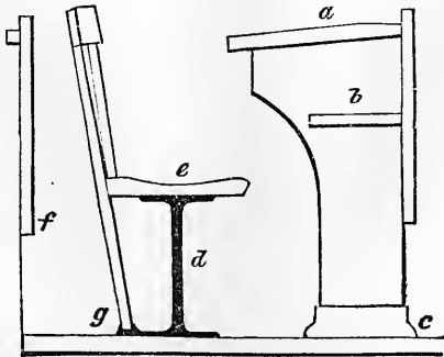
No. 7.—Section of a Writing-Desk and Seat.
