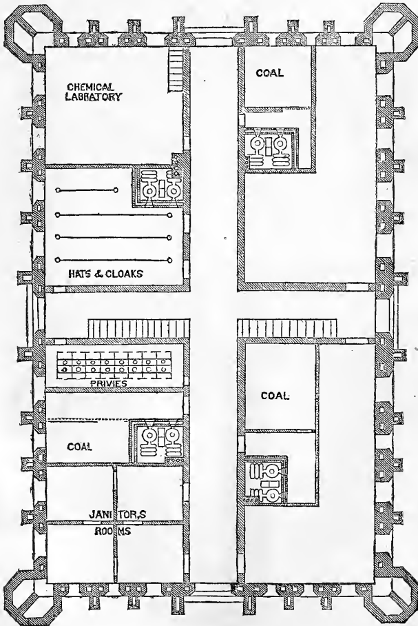
Fig. 3.—BASEMENT FLOOR.
