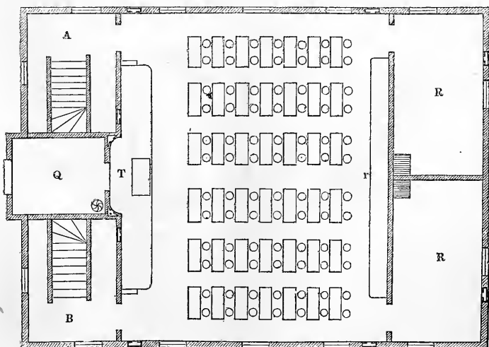
Fig. 4.—SECOND FLOOR.
