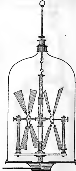
VANE AND MILL IN VACUO Fig. 70.
