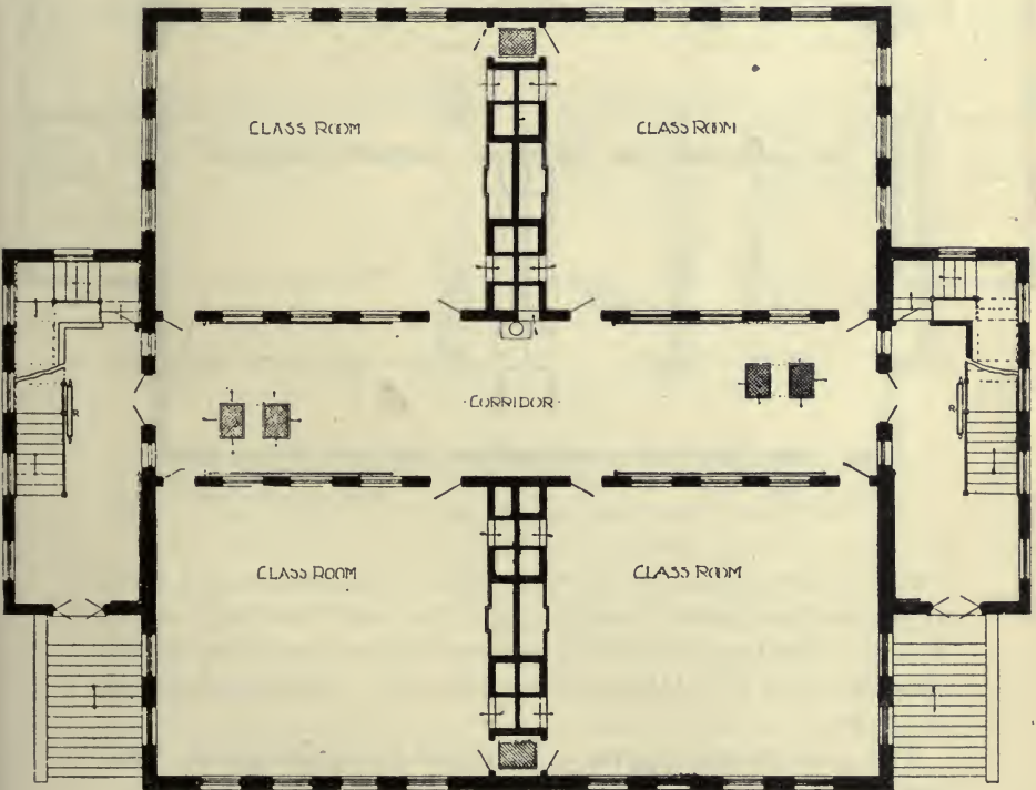
FIRST STORY - SHOWING HEATING & VENTILATIONS EIGHT-ROOM SCHOOL
