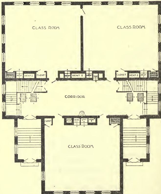
·FIVE ROOM SCHOOL· FIRST STORY·
