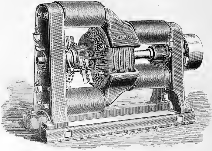
CLARK ELECTRIC COMPANY'S DYNAMO.
