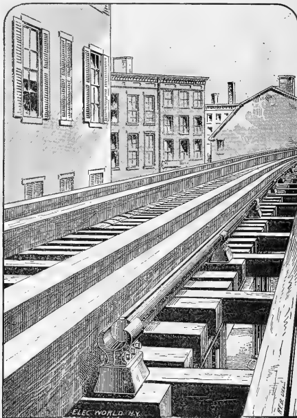
NEW DAFT CONDUCTOR, NEW YORK ELEVATED ROAD.
