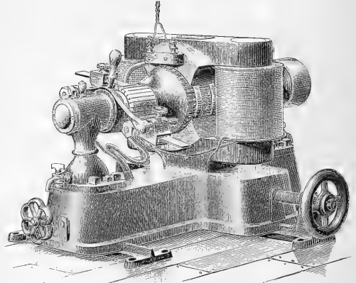
THE DENISON MOTOR AND DYNAMO.
