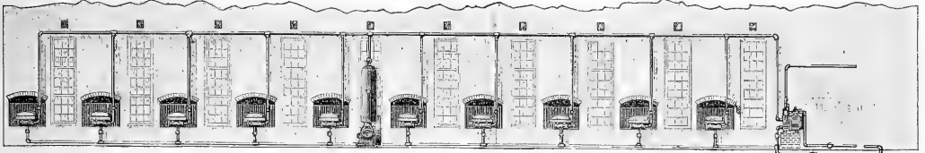
FIG. 1.—FORGES BURNING CRUDE PETROLEUM.
