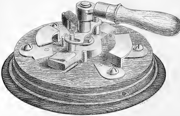
FIG. 4.—DOUBLE-POLE SWITCH.
