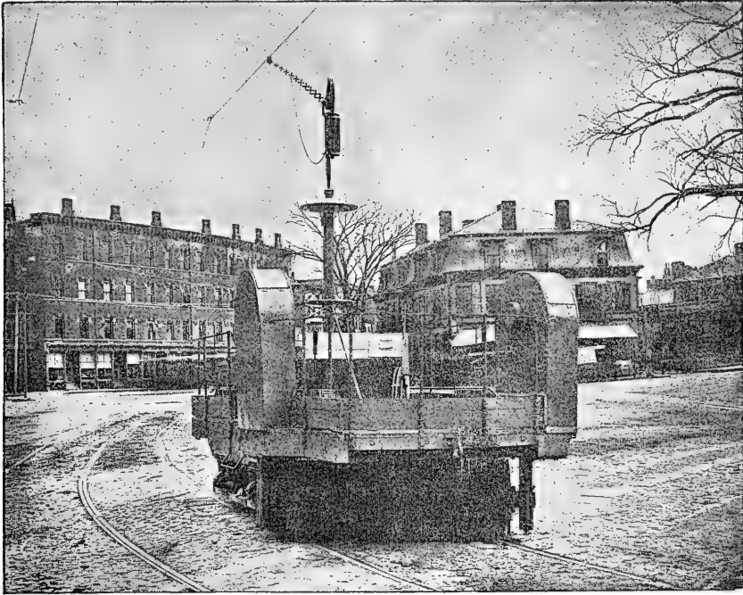
THE THOMSON-HOUSTON SNOW-SWEEPER.
