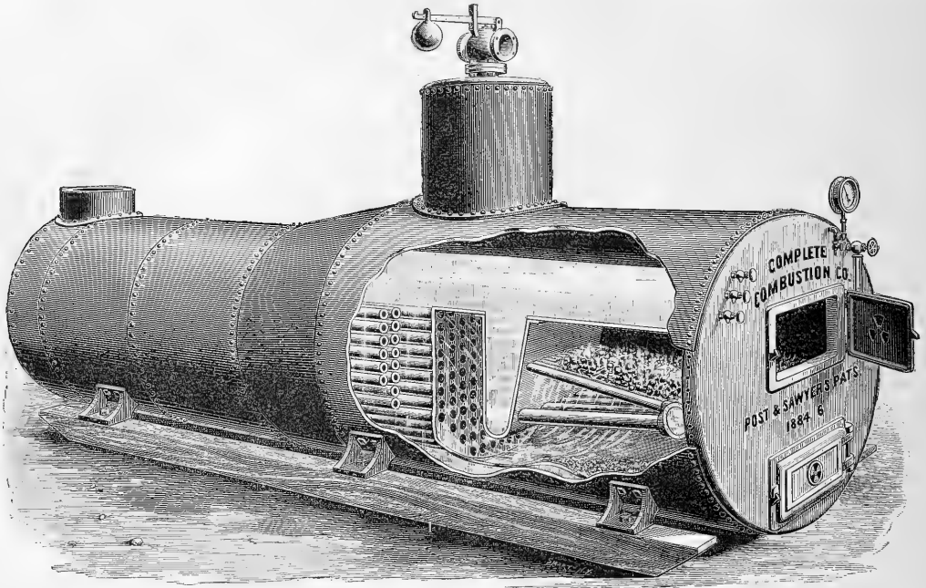
COMPLETE COMBUSTION BOILER.
