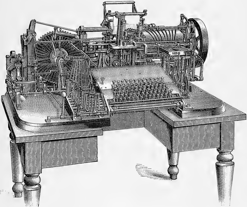
RISLEY AND LAKE COMPOSING-MACHINE.
