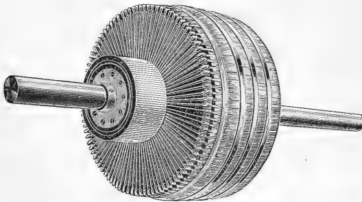
FIGS. 2 AND 3.—ARMATURE OF SPERRY DYNAMO.
