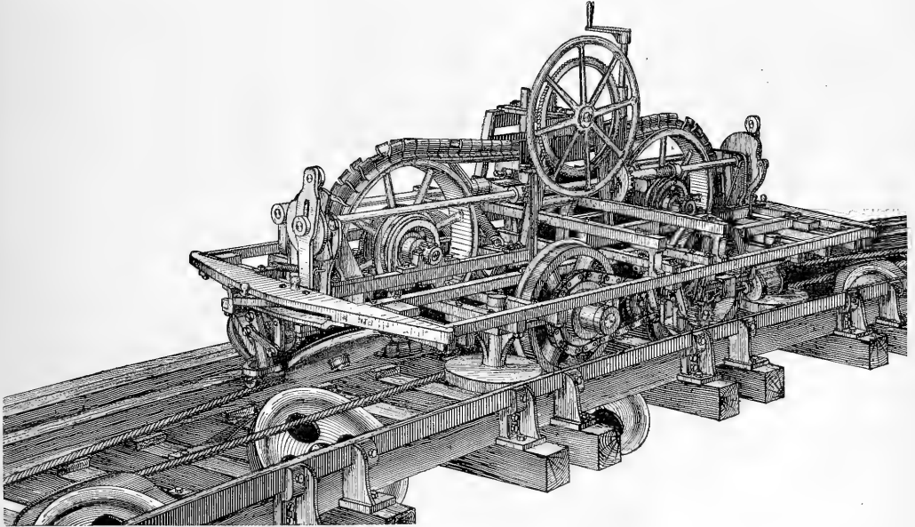
FIG. 2.—MOTOR WITH CAB REMOVED.
