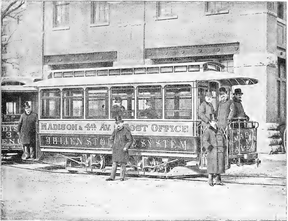
STREET-CAR DRIVEN BY JULIEN STORAGE-BATTERIES.
