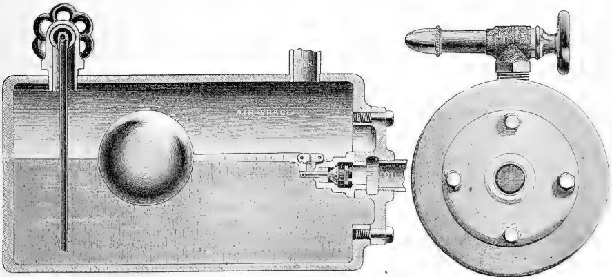
FIG. 2.—AERATING CYLINDER FOR PETROLEUM BURNER.
