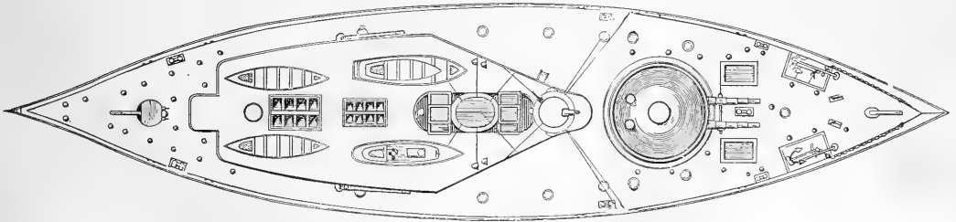
THE SUBMERGING MONITOR CRUISER.
