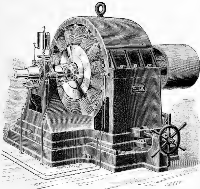
THE WESTINGHOUSE 1500-LIGHT ALTERNATING-CURRENT DYNAMO.
