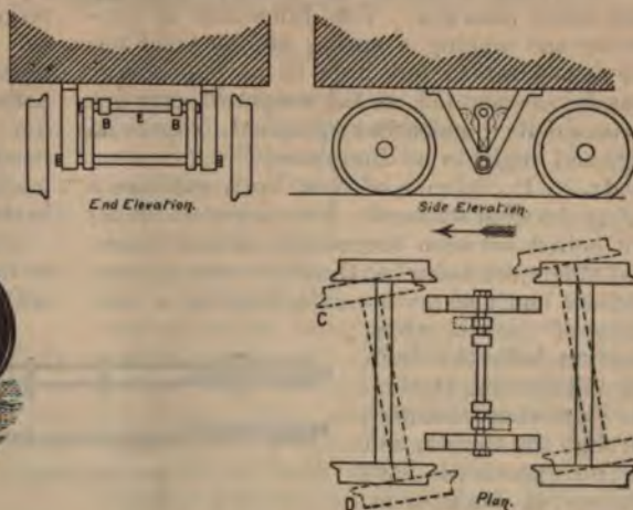
DIAGRAM SHOWING ACTION OF SUSPENSION CAR-TRUCK.
