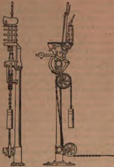
DEVICE FOR KEEPING SIGNAL-WIRE TIGHT.
