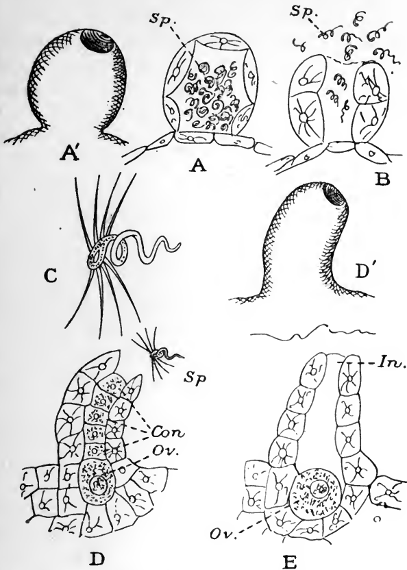
FIG. 9.—The sperm-sacs and egg-pits of the prothallus of the ferns highly magnified. A'. Surface view of a ripe open sperm-sac. A. Section through it, showing the flattened cells forming its walls and the contained corkscrew-like "sperms." B. The minute wriggling sperms ( Sp. ) escaping from the sperm-sac into the water adhering to the surface of the prothallus. C. A single sperm still more magnified. D'. Surface view of an open egg-pit. D. Section through an unfertilised egg-pit. Sp. A sperm swimming towards the open mouth of the egg-pit. Con. Cells forming conducting-plug along which the sperm will travel. Ov. Ovule or egg-cell. E. Fertilised egg-pit. In. The orifice. Ov. The ovule now fertilised and enlarging.
