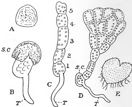
FIG. 7.—Germination of the spore of a fern. A. A single spore about \frac{1}{100} th of an inch in diameter. B. The protoplasm bursts from the spore-coat, S.C. , and sends out a filament-like growth, T . In the third drawing, marked c , this becomes a rooting filament, and the rest has divided into five cells, 1-5, containing chlorophyll grains. D. The front cells are now dividing laterally as well as transversely. E. The prothallus or Marchantia-like growth, twice the natural diameter.
