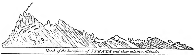
FIG. 23. William Smith's Geological Section across the South of England. Exaggeration of the vertical scale makes the beds appear too steep. The original drawing was in colors. (From Scott, "Land Mammals of Western Hemisphere," published by the Macmillan Co. Reprinted by permission.)
