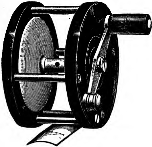
Single Action Click Reel, Rubber, With Protected, Balance Handle.
