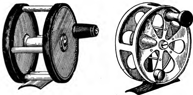
Single Action Reel with Revolving Side Plate and Expert Click Reel.
