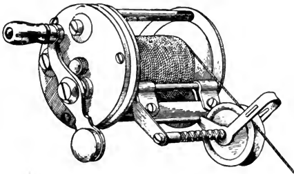
Redifor Reel with Automatic Spooler.
