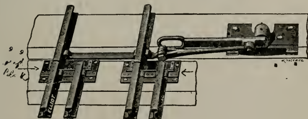
FIG. 115. STUB SWITCH.
