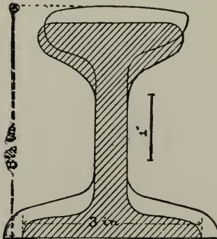
George Stephenson's Fish-Belly Rail, Manchester & Liverpool Railway, A. D. 1829.
