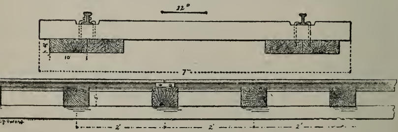
Stevens' Rail, Vicksburg & Jackson Railroad, A. D. 1841
