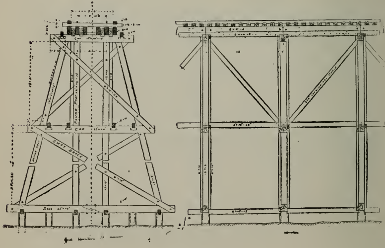
FIG. 167. FRAMED TRESTLE.
