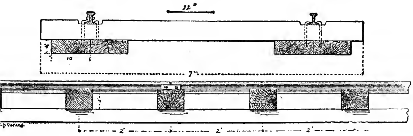
Stevens' Rail, Vicksburg & Jackson Railroad, A. D. 1841
