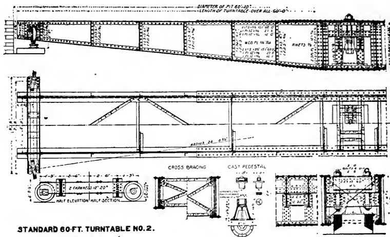
FIG. 184. WROUGHT IRON TURNTABLE. (Made by the King Iron Bridge Co.)
