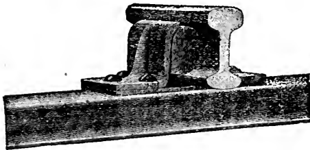
Steel Tie, London & Northwestern Railway, A. D. 1885.
