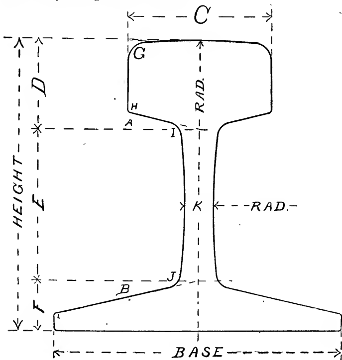
FIG. 379. RAIL SECTION.
