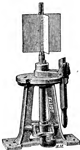
FIG. 139. LOW PONY SWITCH STAND WITH SAFETY BOTTOM CAP.
