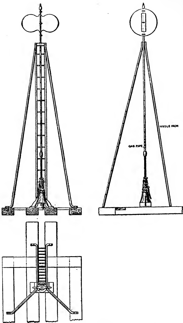
FIG. 142. TARGET TRIPOD FOR SWITCH STANDS.
