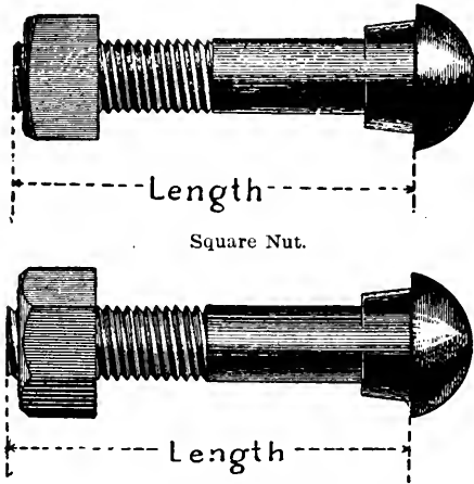
FIG. 109. TRACK BOLTS.
