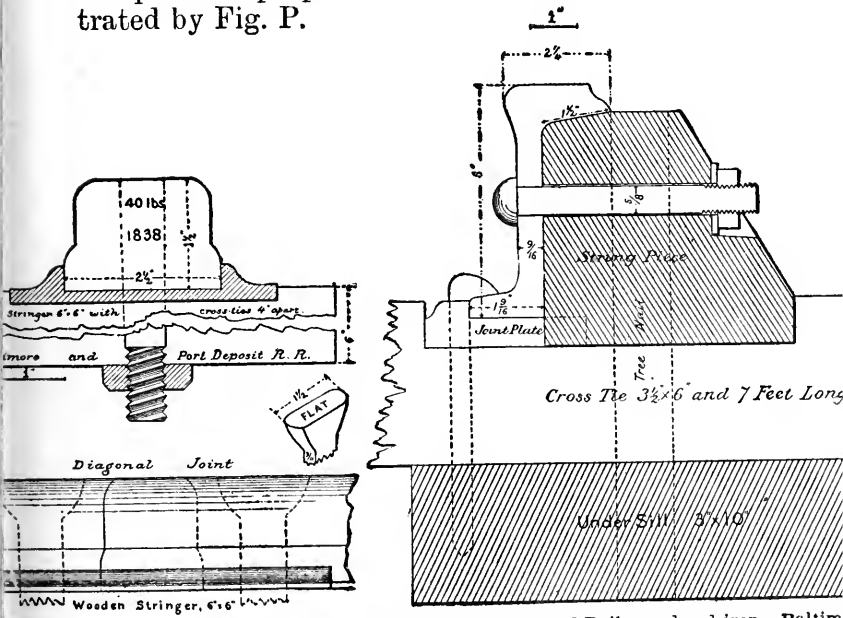
Thick Rectangular Rail, A. D. 1838.
