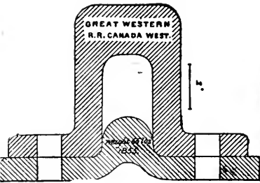
Box Rail.
