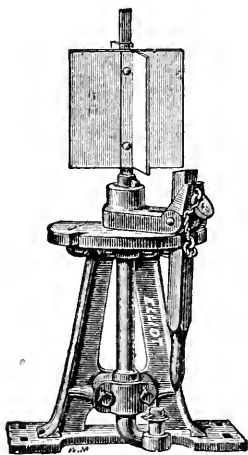
FIG. 138. LOW PONY SWITCH STAND.
