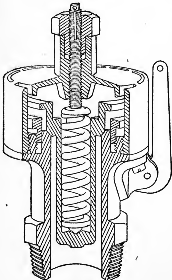
FIG. 29. SECTIONAL VIEW OF POP VALVE.
