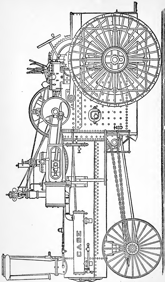
FIG. 1. LEFT SIDE ELEVATION OF "CASE" TRACTION ENGINE.
