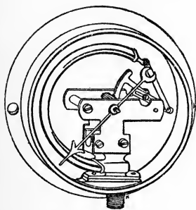
FIG. 27. INTERIOR OF GAGE.
