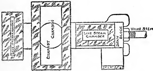
FIG. 19. FACE OF VALVE.
