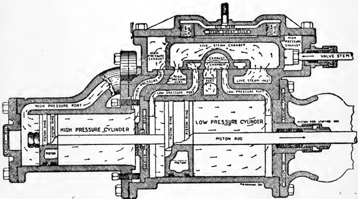
FIG. 18. SECTIONAL VIEW OF "WOOLF" COMPOUNDED CYLINDER.
