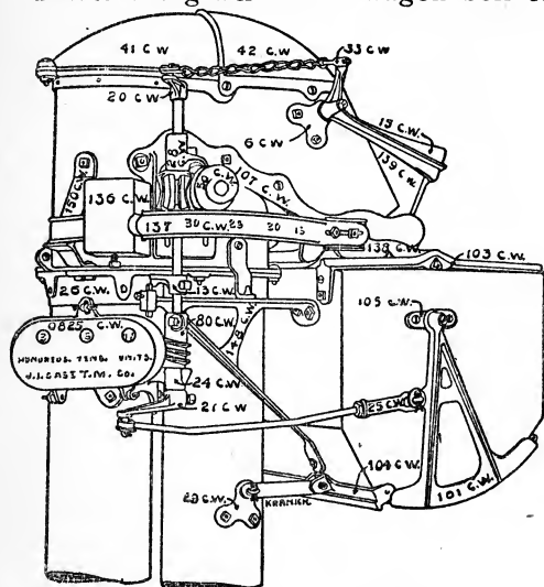
FIG. 49. HEAD OF CASE WEIGHER.
