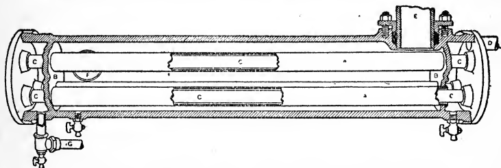
FIG. 5. SECTIONAL VIEW OF "CASE" HEATER.
