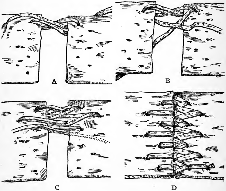
FIG. 52. STITCHED CANVAS BELT LACINGS
