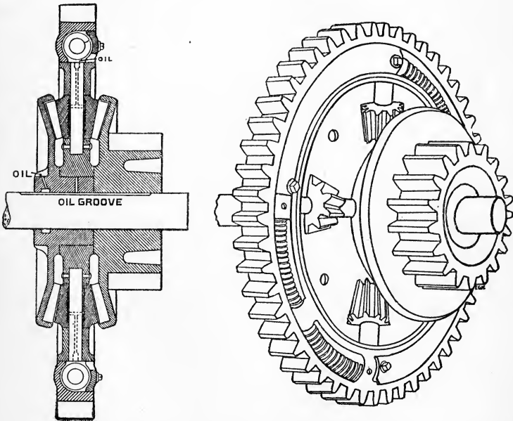
FIG. 34. THE DIFFERENTIAL GEAR, SHOWING SPRINGS
