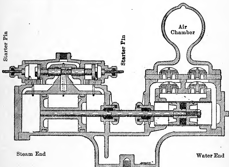
FIG. 3. SECTIONAL VIEW OF MARSH PUMP.
