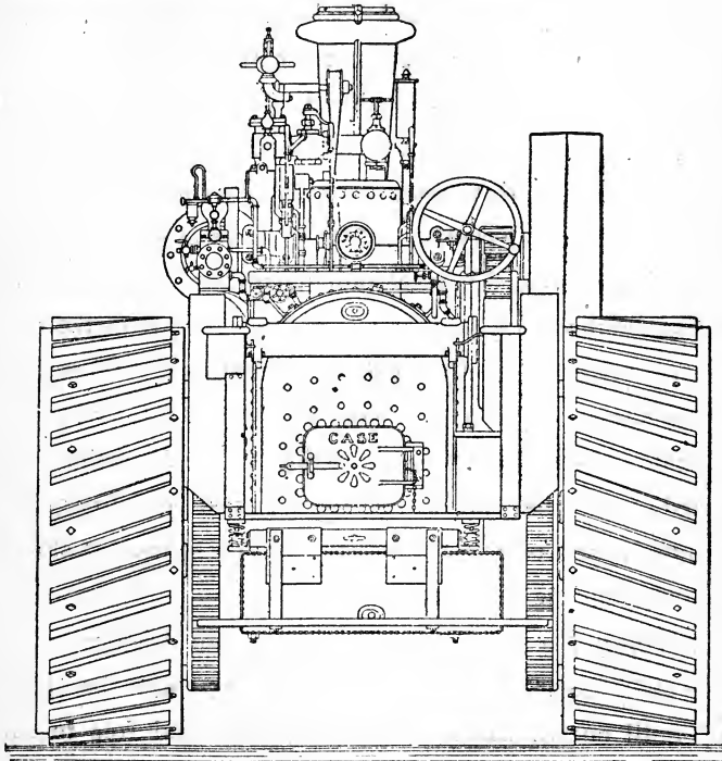
FIG. 33. REAR VIEW OF "CASE" TRACTION ENGINE.
