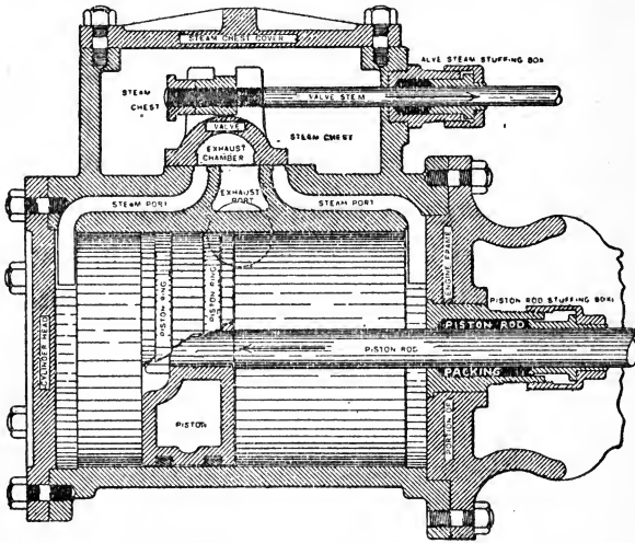
FIG. 15. SECTIONAL VIEW OF SIMPLE CYLINDER.
