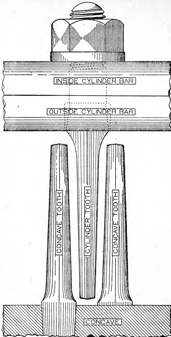
FIG. 39. CUT SHOWING SPACE BETWEEN CYLINDER AND CONCAVE TEETH—FULL SIZE.
