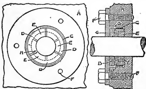
FIG. 21. THE CENTER-HEAD PACKING.
