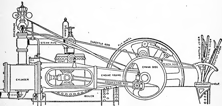
FIG. 14. SIDE ELEVATION OF ENGINE PROPER.
