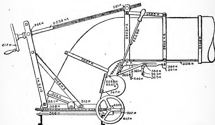
FIG. 48. TELESCOPING DEVICE FOR STRAW-CHUTE.
