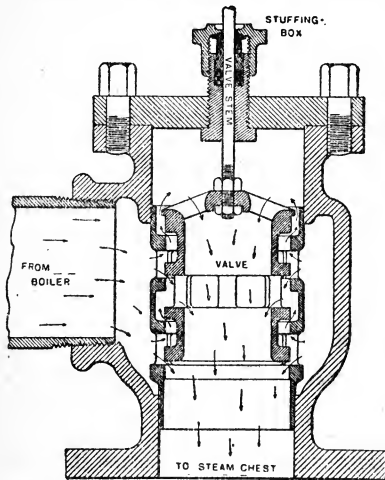
FIG. 17. SECTION OF GOVERNOR VALVE
