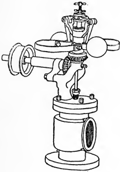
FIG. 16. GOVERNOR.
