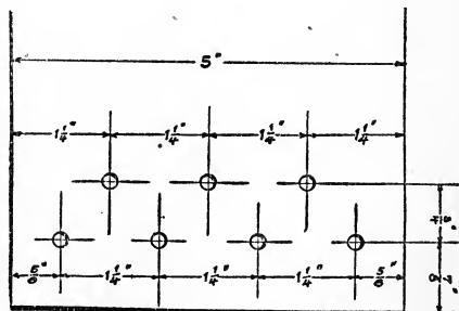
FIG. 51. LOCATION OF HOLES FOR LACING CANVAS BELT.
