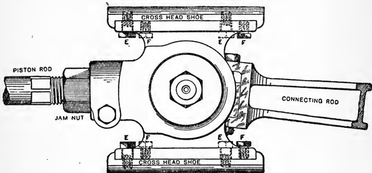
FIG. 12. THE CROSS-HEAD.
