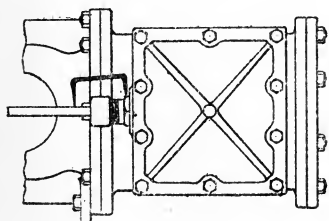
FIG. 25. TRAM ON VALVE-STEM.
