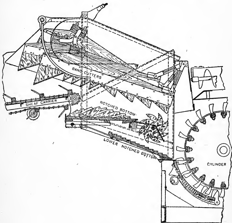
FIG. 45. SECTIONAL VIEW OF "CASE" FEEDER.
