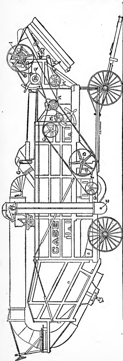
FIG. 44. LEFT SIDE OF SEPARATOR WITH FEEDER AND WIND STACKER.
