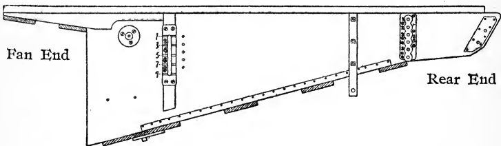
FIG. 41. SHOE SHOWING POSITIONS OF SIEVE RODS.
