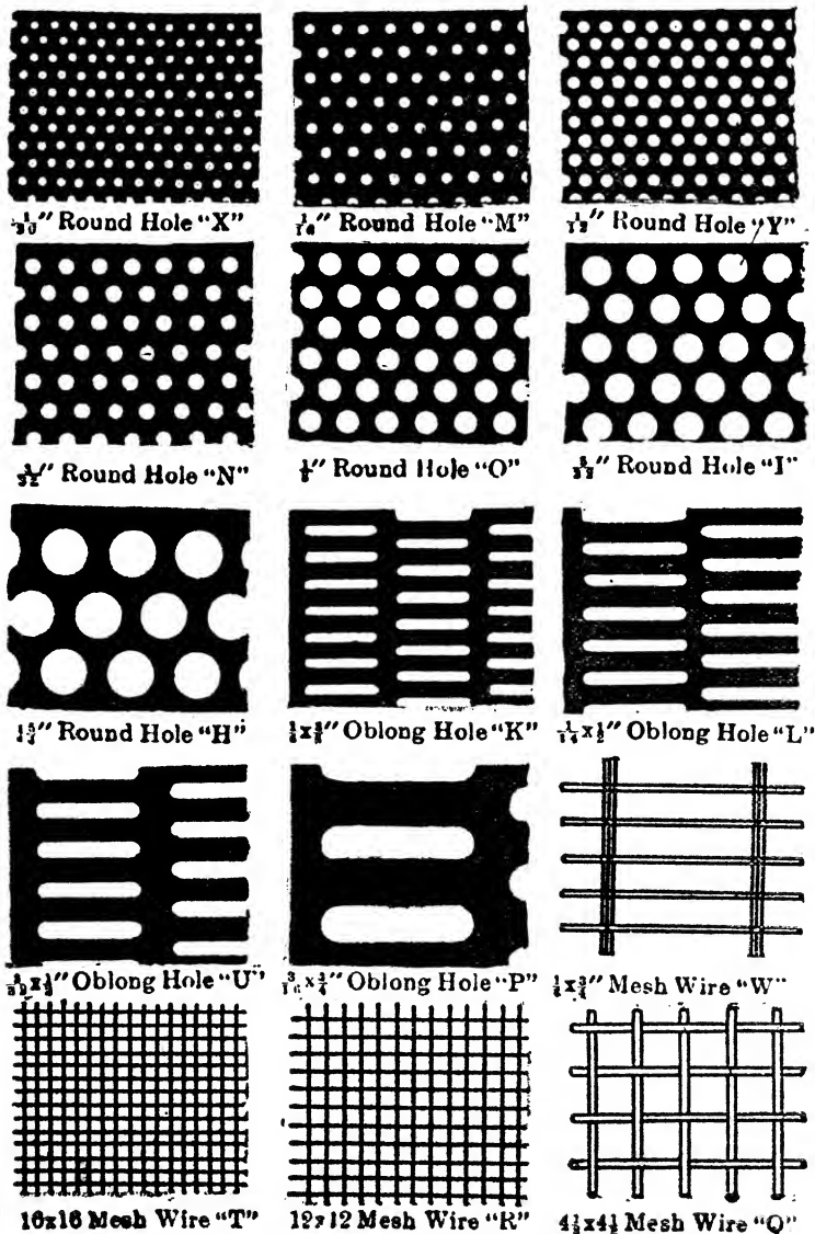
FIG. 43. SIEVES AND SCREENS. (Full Size.)
