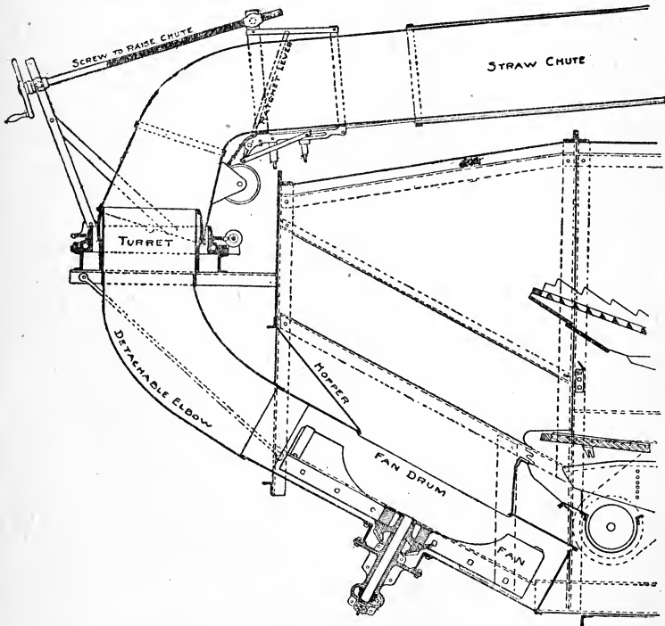
FIG. 47. SECTIONAL VIEW OF WIND STACKER.
