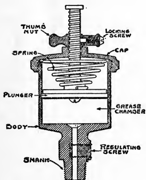
FIG. 8. SECTIONAL VIEW OF "IDEAL" CUP.
