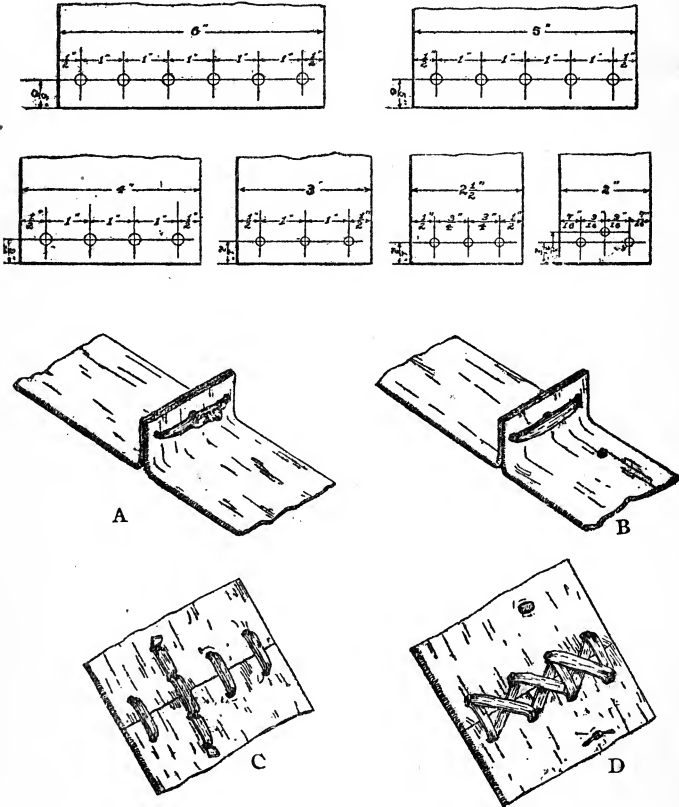
FIG. 50. LEATHER BELT LACINGS.
