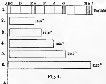
Fig. 4. Spectra of daylight and of incandescent platinum at different temperatures.
