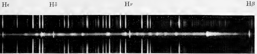
FIG. 21. SPECTRUM OF WOLF-RAYET STAR, PLANETARY NEBULA, B. D. +30.°3639. Photographed at the Lick Observatory.
