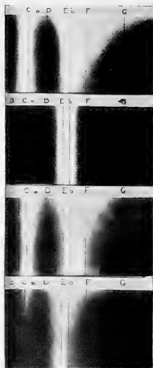
The spectra of solutions of Chromium Salts at different temperatures.
