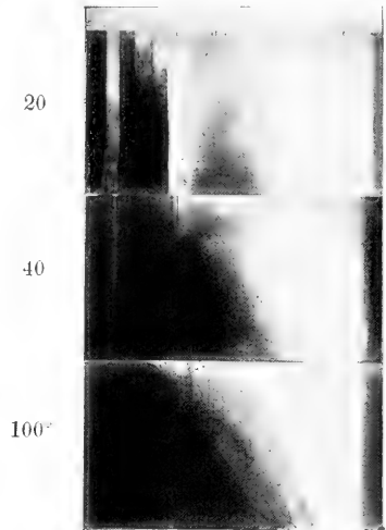
C. Spectra at different temperatures of a saturated solution of Cobalt Chloride mixed with a saturated solution of Calcium Chloride.
