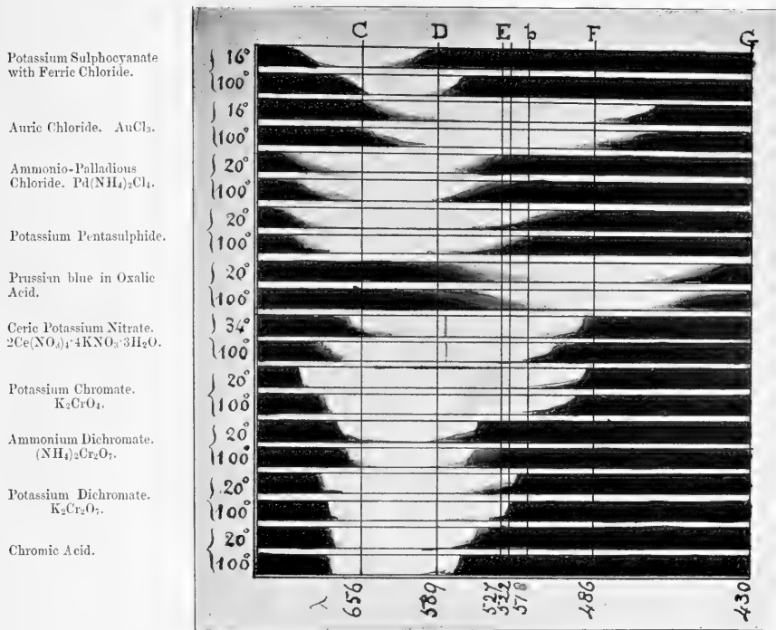
The Absorption Spectra of solutions of various Anhydrous Salts at different temperatures. These show no marked alteration when heated.
