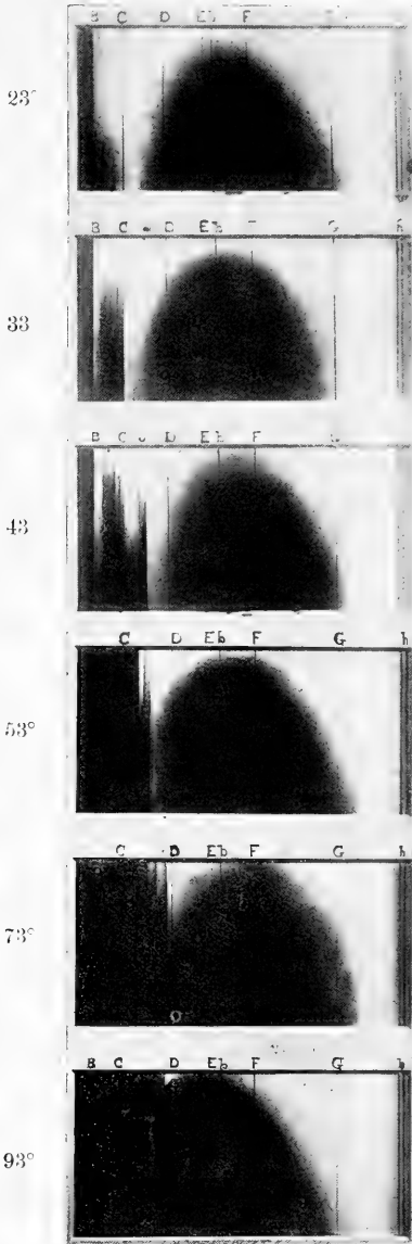
A. Spectra of saturated aqueous solution of Cobalt Chloride at different temperatures, showing dissociation of the molecules of Water from the Metallic Chloride.
