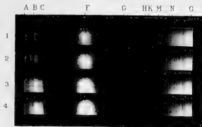
RED POTASSIUM CHROMALATE AT DIFFERENT TEMPERATURES NAMELY: 1 AT 100°, 2 AT 75°, 3 AT 50° AND 4 AT 20° C
