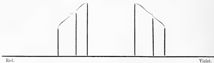
FIG. 8.—TRIPLLET OF SECOND SERIES. FIG. 9.—TRIPLLET OF FIRST SERIES. [The ordinates represent the separations \delta\lambda of the side lines by the same magnetic field.]
