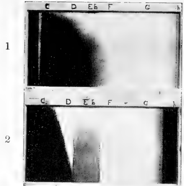
B. 1. Anhydrous Cobalt Chloride dissolved in Alcohol. 2. Solution of Cobalt Chloride mixed with Hydrochloric Acid. (Both solutions are unaltered by heat.)
