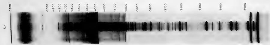
BANDED FLAME SPECTRA OF METALS.
