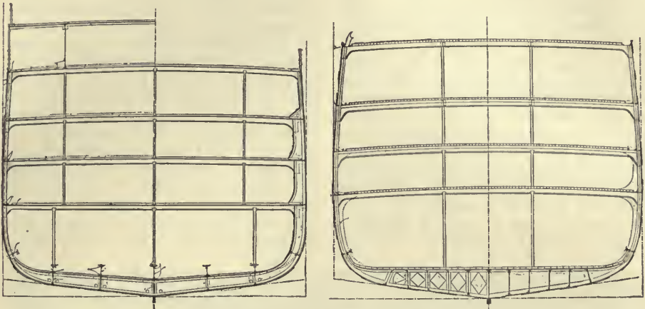
Cross-sections of the Oregon and Servia.
