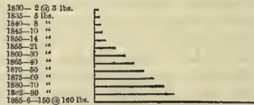
Diagram showing Increase in Steam-pressures based on good Average Practice.
