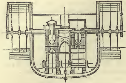
Cross-section of the Great Western.
