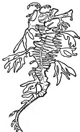
FIG. 19.— Phyllopteryx eques , a sea-horse ( \times \frac{2}{3} ).
