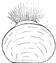
FIG. 30. Larva of Shipworm (Teredo) greatly enlarged.
