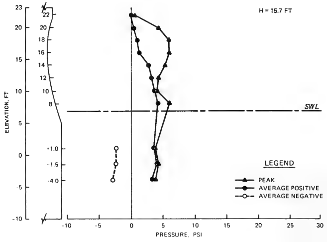
DISTRIBUTION OF WAVE PRESSURES PLAN R4S2 SWL = +6.9 FT, T = 10 SEC H = 14.7 AND 15.7 FT
