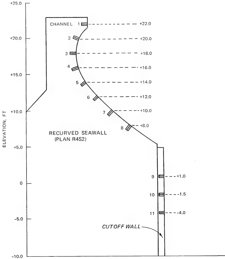
Figure 4. Pressure transducer locations on recurved seawall
