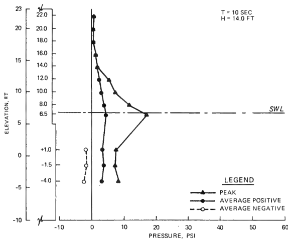
DISTRIBUTION OF WAVE PRESSURES PLAN R4S1 SWL = +6.9 FT T = 8 AND 10 SEC H = 13.4 AND 14.0 FT
