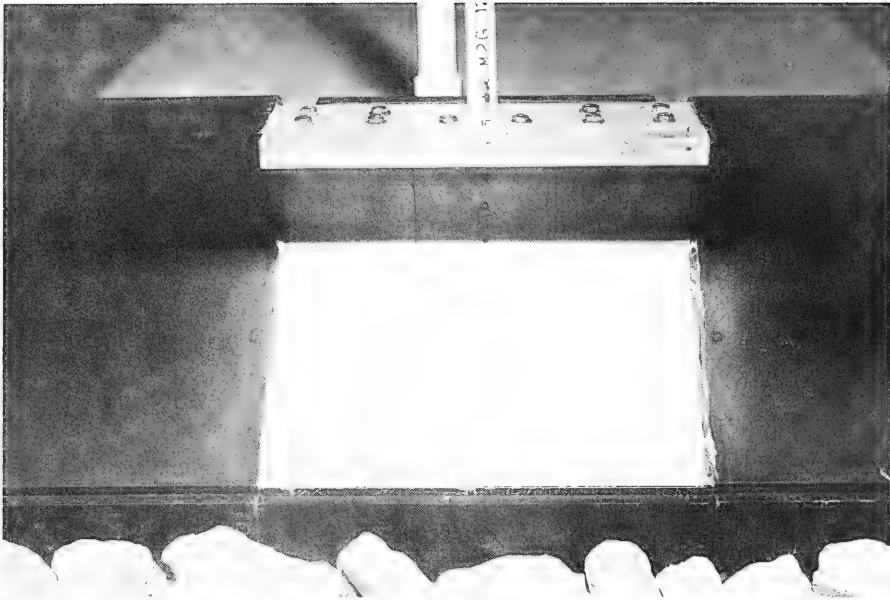
Figure 11. Sea-side view of instrumented recurved seawall face for a 14-sec, 11.4-ft breaking wave at an swl of 8.6 ft msl. Average secondary wave pressures on the modified recurved seawall are listed in Table 7.
