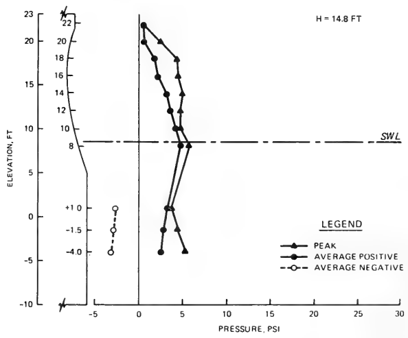
DISTRIBUTION OF WAVE PRESSURES PLAN R4S2 SWL = +8.6 FT, T = 10 SEC H = 12.1 AND 14.8 FT
