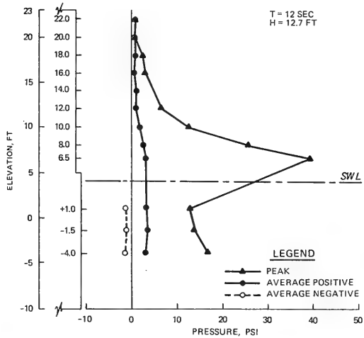
DISTRIBUTION OF WAVE PRESSURES PLAN R4S1 SWL = +4.3 FT T = 10 AND 12 SEC H = 12.8 AND 12.7 FT
