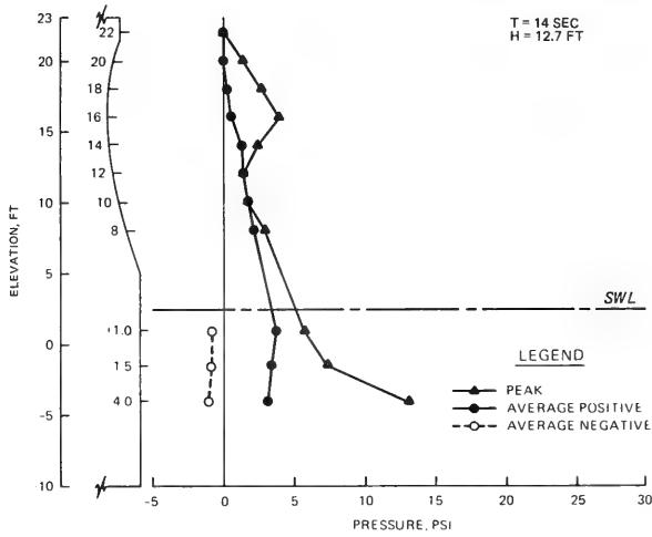
DISTRIBUTION OF WAVE PRESSURES PLAN R4S2 SWL = + 2.6 FT T = 12 AND 14 SEC H = 12.6 AND 12.7 FT
