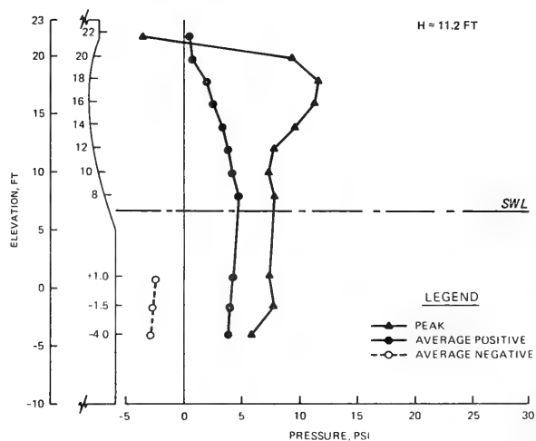
DISTRIBUTION OF WAVE PRESSURES PLAN R4S2 SWL = +6.9 FT, T = 14 SEC H = 16.3 AND 11.2 FT
