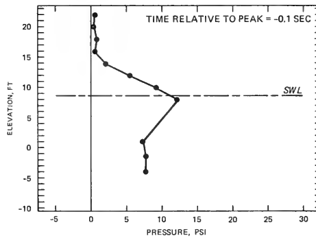
INSTANTANEOUS WAVE PRESSURE DISTRIBUTION PLAN R4S2 SWL = +8.6 FT, T = 14 SEC, H = 11.4 FT TIME INCREMENT = -0.5 TO -0.1 SEC
