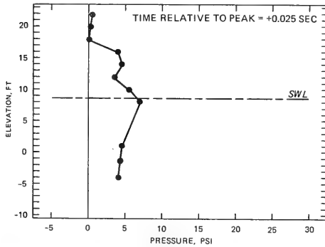
INSTANTANEOUS WAVE PRESSURE DISTRIBUTION PLAN R4S2 SWL = +8.6 FT, T = 12 SEC, H = 16.8 FT TIME INCREMENT = -0.025 TO +0.025 SEC
