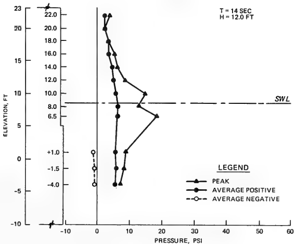
DISTRIBUTION OF WAVE PRESSURES PLAN R4S1 SWL = +8.6 FT T = 12 AND 14 SEC H = 16.0 AND 12.0 FT
