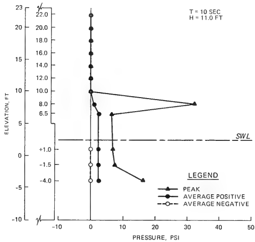
DISTRIBUTION OF WAVE PRESSURES PLAN R4S1 SWL = +2.6 FT T = 8 AND 10 SEC H = 11.1 AND 11.0 FT
