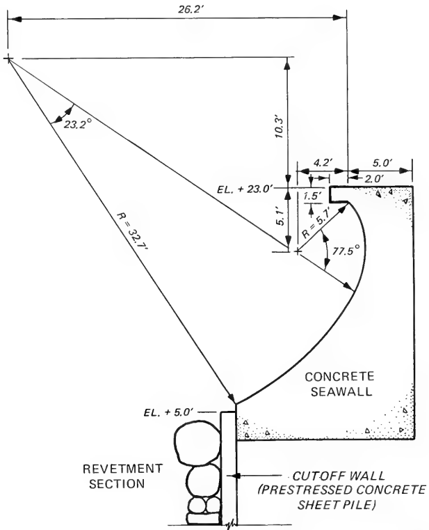
Figure 7. Details of seawall curvature, Plan R4S3
