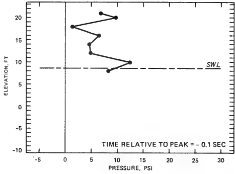
INSTANTANEOUS WAVE PRESSURE DISTRIBUTION PLAN R4S3 SWL = +8.6 FT T = 14 SEC, H = 11.4 FT TIME INCREMENT = -0.5 TO -0.1 SEC
