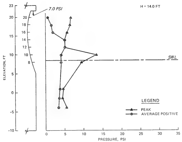
DISTRIBUTION OF WAVE PRESSURES PLAN R4S3 SWL = +8.6 FT, T = 12 SEC H = 12.0 AND 14.0 FT
