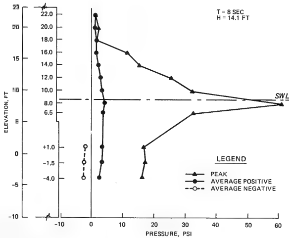
DISTRIBUTION OF WAVE PRESSURES PLAN R4S1 SWL = +8.6 FT T = 6 AND 8 SEC H = 12.5 AND 14.1 FT
