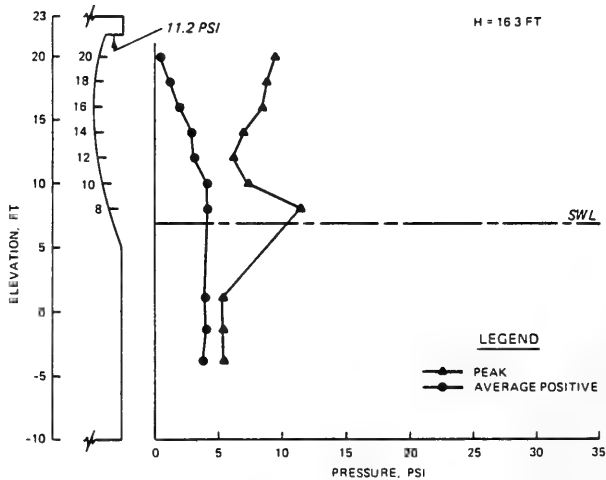
DISTRIBUTION OF WAVE PRESSURES PLAN R4S3 SWL = +6.9 FT, T = 14 SEC H = 14.0 AND 16.3 FT
