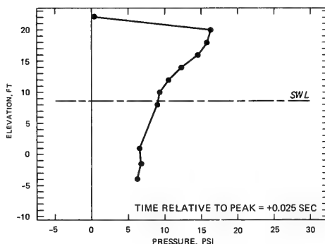
INSTANTANEOUS WAVE PRESSURE DISTRIBUTION PLAN R4S2 SWL = +8.6 FT, T = 14 SEC, H = 17.0 FT TIME INCREMENT = -0.025 TO +0.025 SEC
