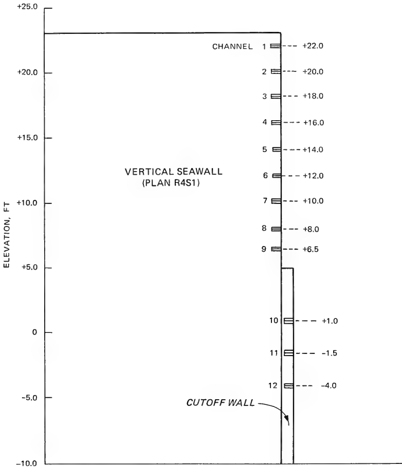
Figure 3. Pressure transducer locations on vertical seawall
