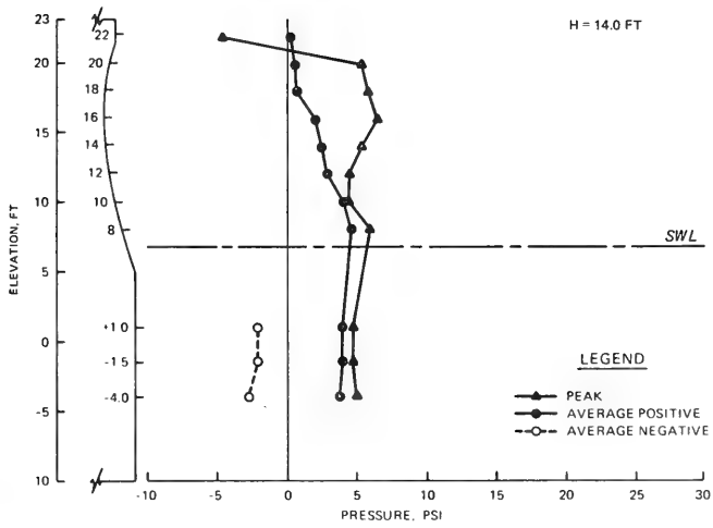
DISTRIBUTION OF WAVE PRESSURES PLAN R4S2 SWL = +6.9 FT, T = 14 SEC H = 12.0 AND 14.0 FT
