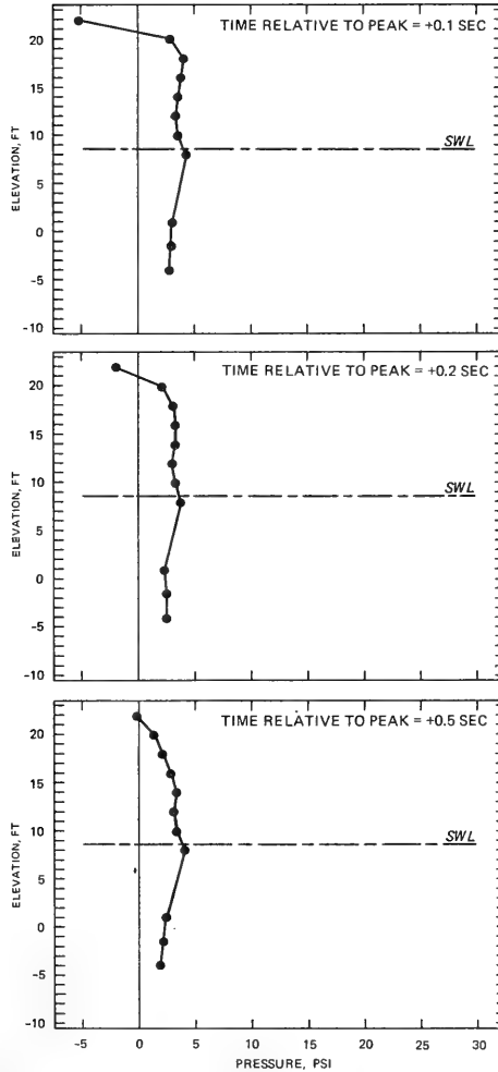
INSTANTANEOUS WAVE PRESSURE DISTRIBUTION PLAN R4S2 SWL = +8.6 FT, T = 12 SEC, H = 12.0 FT TIME INCREMENT = +0.1 TO +0.5 SEC
