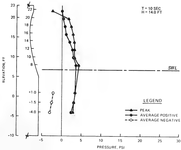
DISTRIBUTION OF WAVE PRESSURES PLAN R4S2 SWL = +6.9 FT T = 8 AND 10 SEC H = 13.4 AND 14.0 FT
