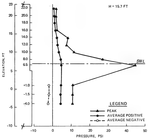
DISTRIBUTION OF WAVE PRESSURES PLAN R4S1 SWL = +6.9 FT, T = 10 SEC H = 14.7 AND 15.7 FT
