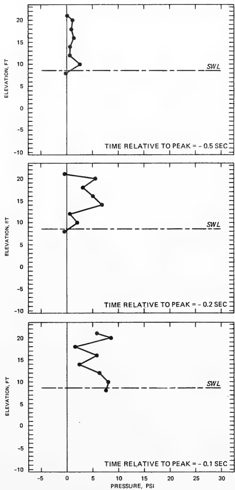
INSTANTANEOUS WAVE PRESSURE DISTRIBUTION PLAN R4S3 SWL = +8.6 FT, T = 14 SEC, H = 17.0 FT TIME INCREMENT = -0.5 TO -0.1 SEC
