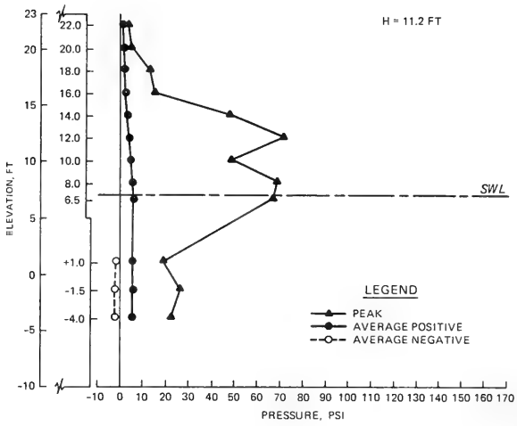
DISTRIBUTION OF WAVE PRESSURES PLAN R4S1 SWL = +6.9 FT, T = 14 SEC H = 16.3 AND 11.2 FT
