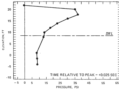
INSTANTANEOUS WAVE PRESSURE DISTRIBUTION PLAN R4S2 SWL = +8.6 FT, T = 14 SEC, H = 11.4 FT TIME INCREMENT = -0.025 SEC TO +0.025 SEC
