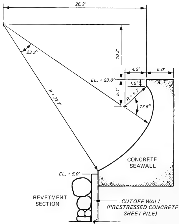
Figure 6. Details of seawall curvature, Plan R4S2
