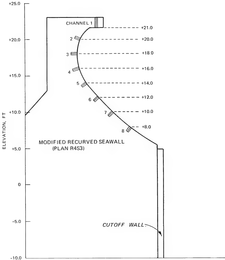
Figure 5. Pressure transducer locations on modified recurved seawall
