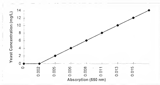
Figure 1. Standard yeast concentration curve for ALCOA pore water assays.
