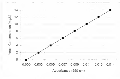
Figure 1. Standard yeast concentration curve for Sylvan Slough porewater assays.
