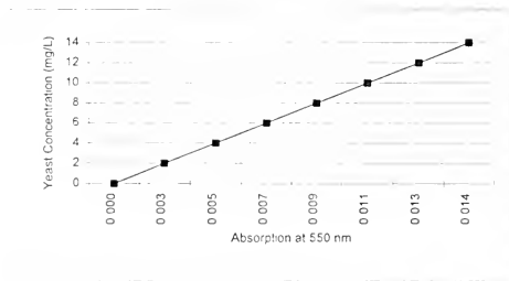
Figure 1 Standard yeast concentration curve for Campbell's Slough porewater assay.
