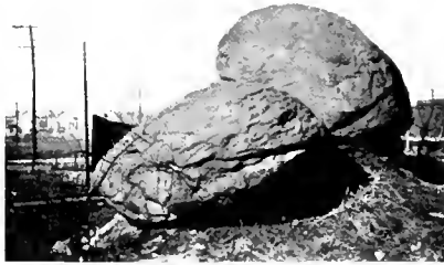
Weathering Balto Gneiss
