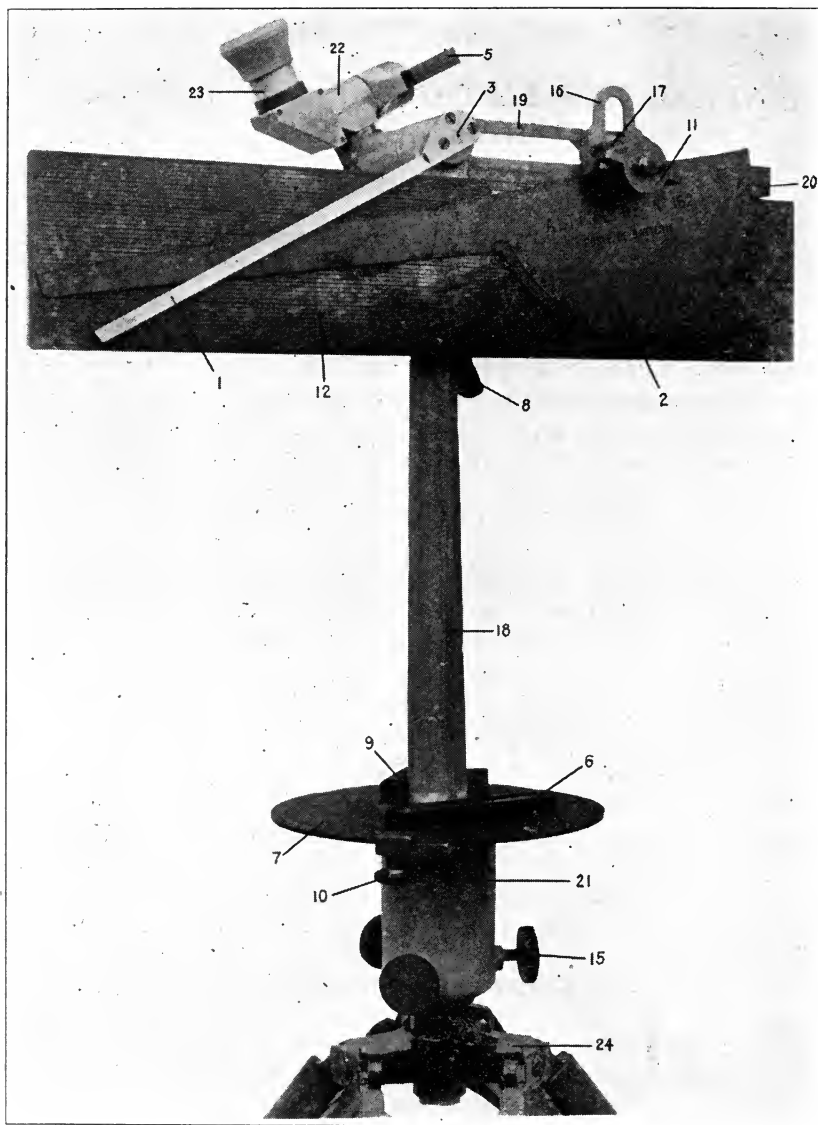
ALTIMETER, MODEL OF 1916. Battery Commander's Station Instrument.
