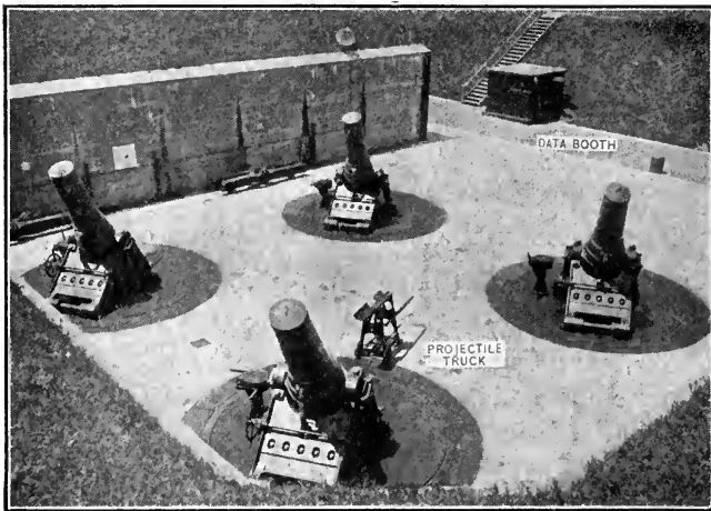
FIG. 11.—Pit of 12-inch Mortars.
