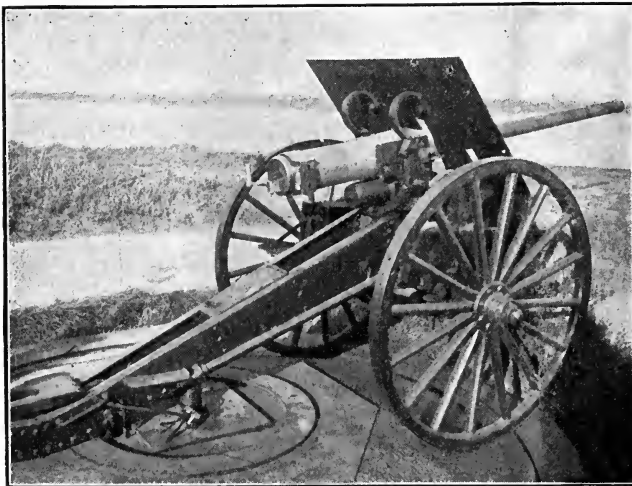
FIG. 16.—2.24-inch (6-pounder) R. F., D.-S. Gun, M. 1900. Interrupted Thread Breech Mechanism. Mounted on Wheeled Mount.
