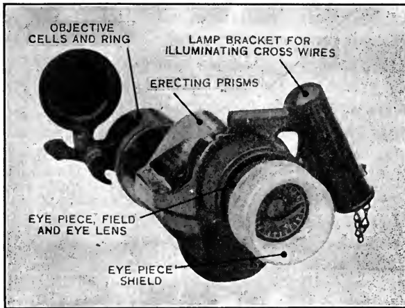
FIG. 59A.—2-inch Telescopic Sight, M. 1906, for 3-inch R.-F. Guns.
