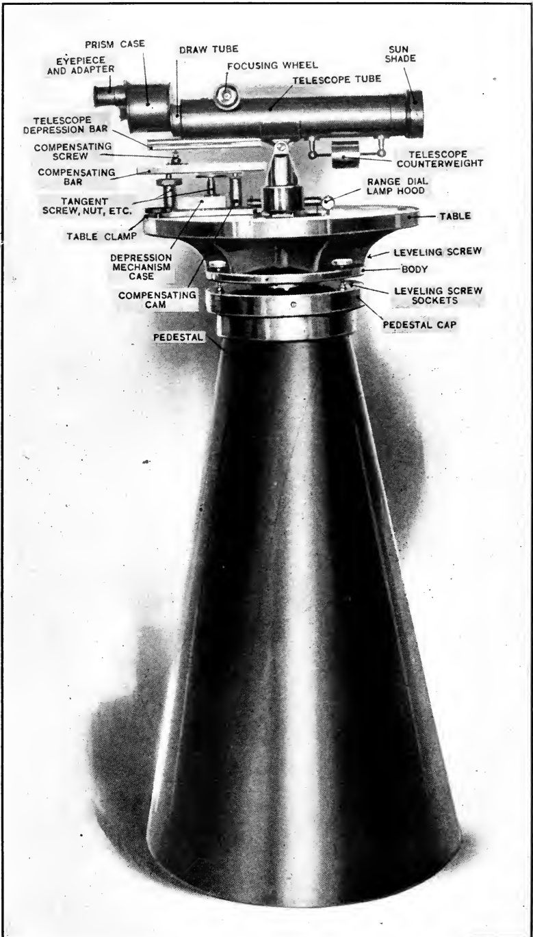
Depression Position Finder, Lewis Type.
