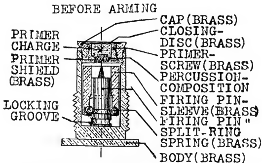
FIG. 38.—Ring Resistance Base Percussion Fuse. For minor calibers.
