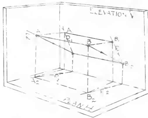
FIGURE 14 SHADOWS OF LINES PARALLEL TO ELEVATION PLANE
