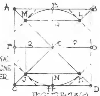
CIRCLE IN PLANE PERPENDICULAR TO PLANE ON WHICH SHADOW IS CAST.
