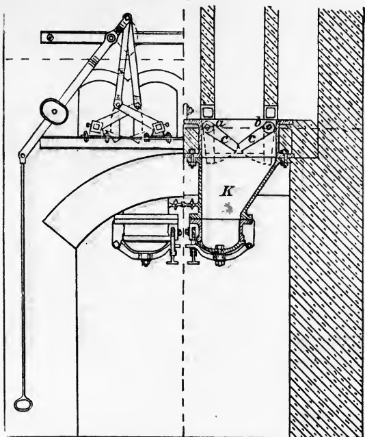
FIG. 25.—Device for discharging spent shale.
