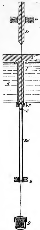
FIG. 62.—Candle Machine.
