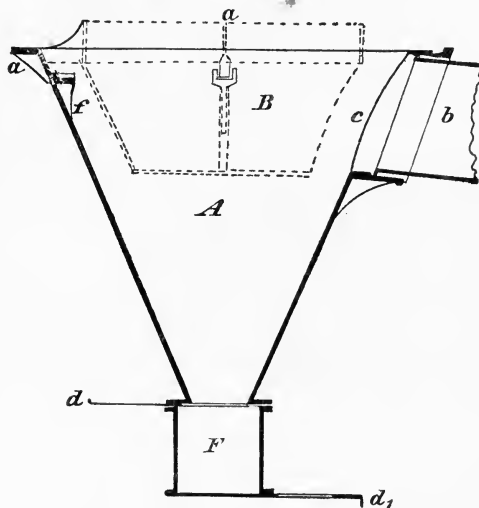
FIG. 9.—Cone and bell of Rolle retort.
