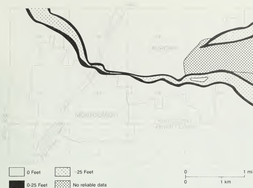
Figure 8 Areal distribution and thickness of sand and gravel deposits in buried bedrock valleys (lower sand and gravel aquifer).
