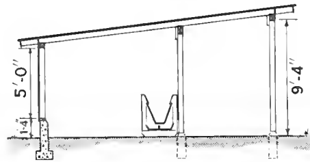
CROSS SECTION
