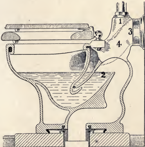
FIG. 18. — Cross section of a siphon water-closet.
