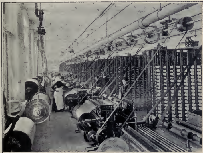
FIG. 57. — Warping in preparation for weaving. The creel holds the spools.
