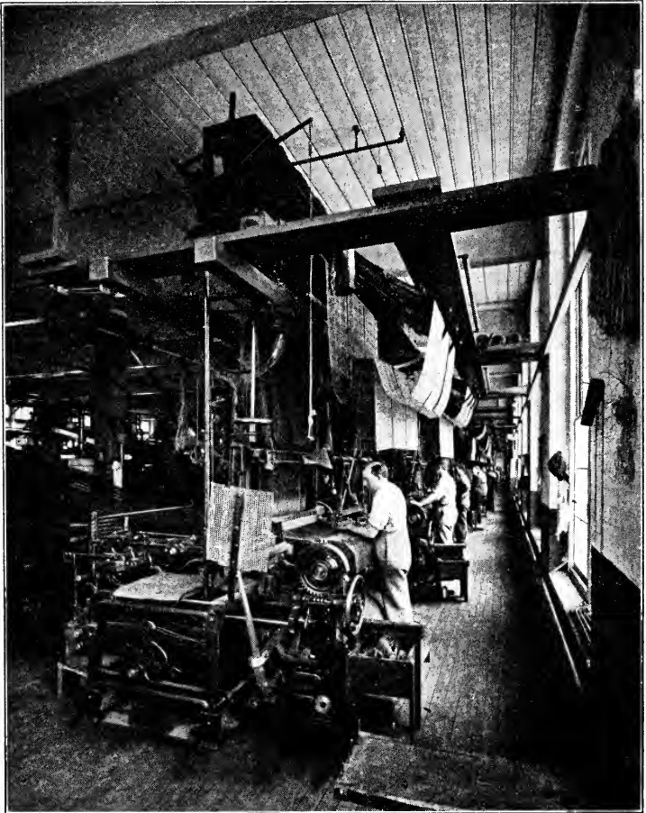
FIG. 73. — This shows the Jacquard loom used for weaving rugs and carpets.
