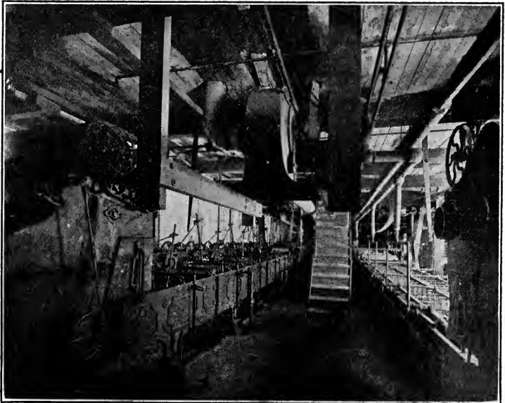
FIG. 66. — Wool washing or scouring. Notice the rakes in the machines which move the wool back and forth in scouring.
