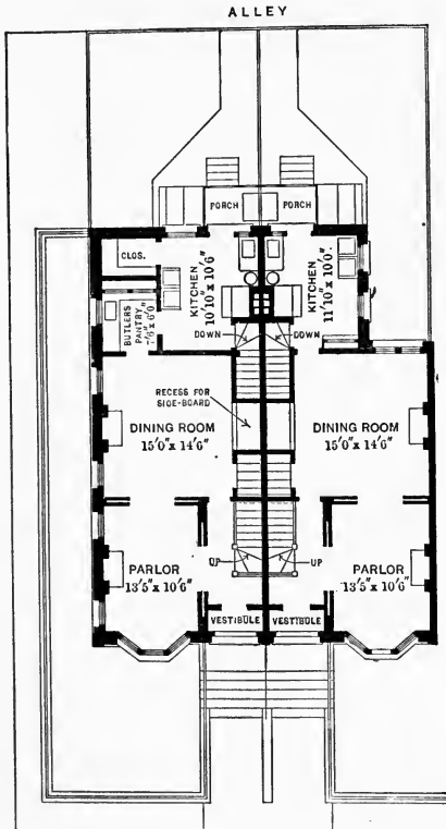
The Morris Building Company's Block of Single Houses, with Central Heating Plant, Brooklyn, New York.
