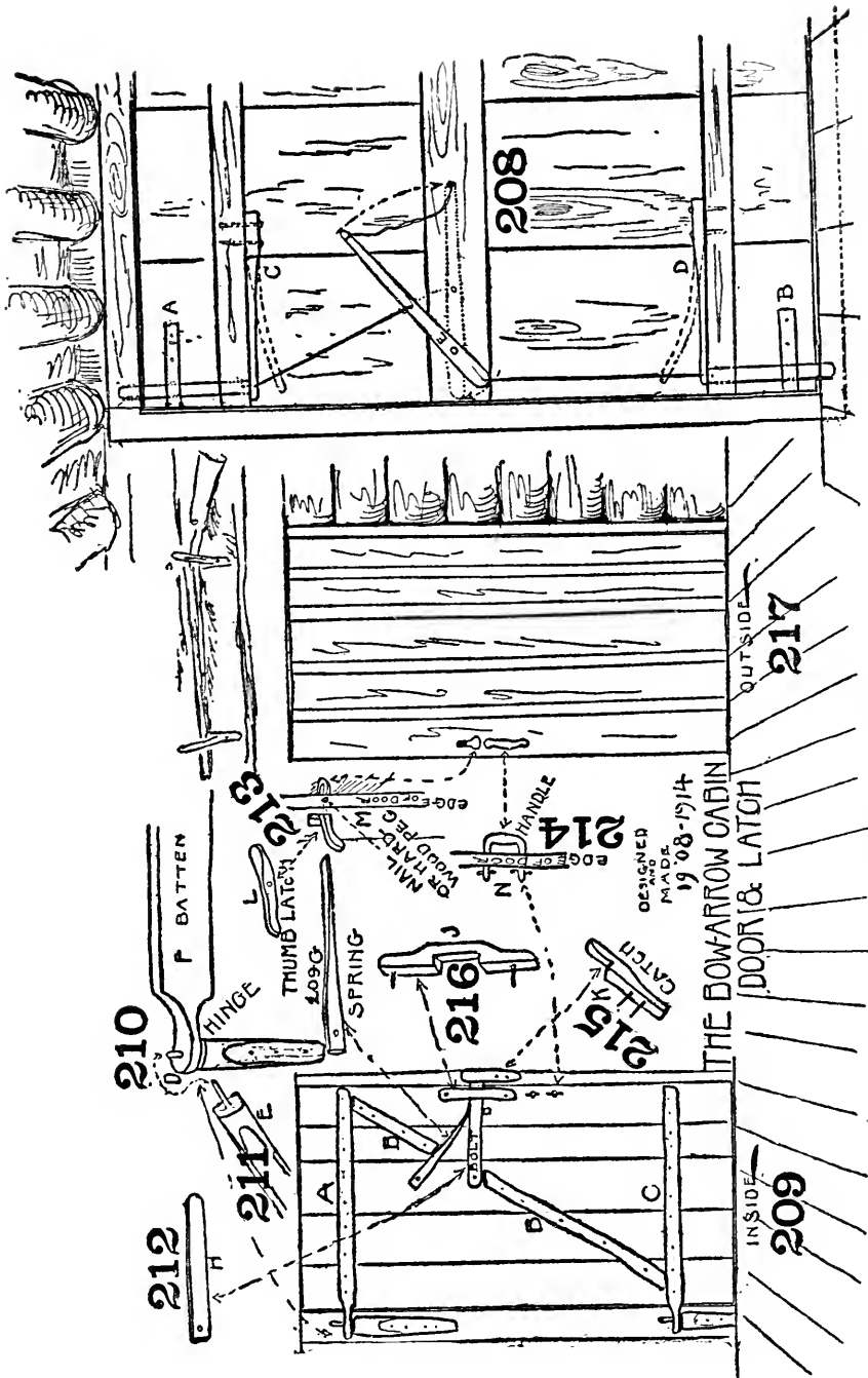
Jack-knife latches suitable for Canada and America.
