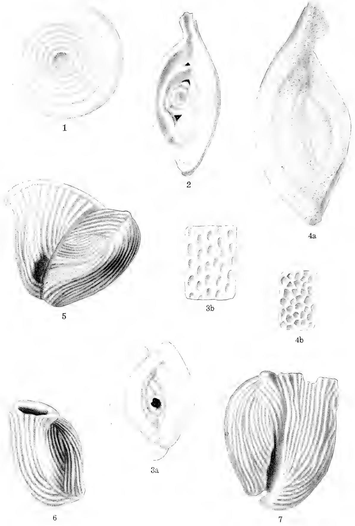
FORAMINIFERA OF THE BRYAM MARL.
