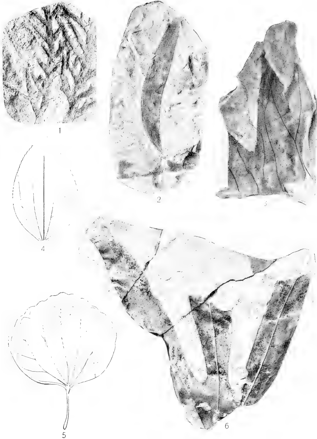
1, Brachyphyllum macrocarpum formosum Berry; 2, Podozamites lanceolatus (Lindley and Hutton) F. Braun; 3, Liriodendron quercifolium Newberry; 4, Zizyphus lamarensis Berry; 5, Trochodendroides rhomboideus Berry; 6, Sterculia lugubris Lesquereux.
