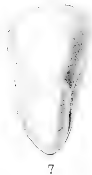
FORAMINIFERA OF THE BYRAM MARL.
