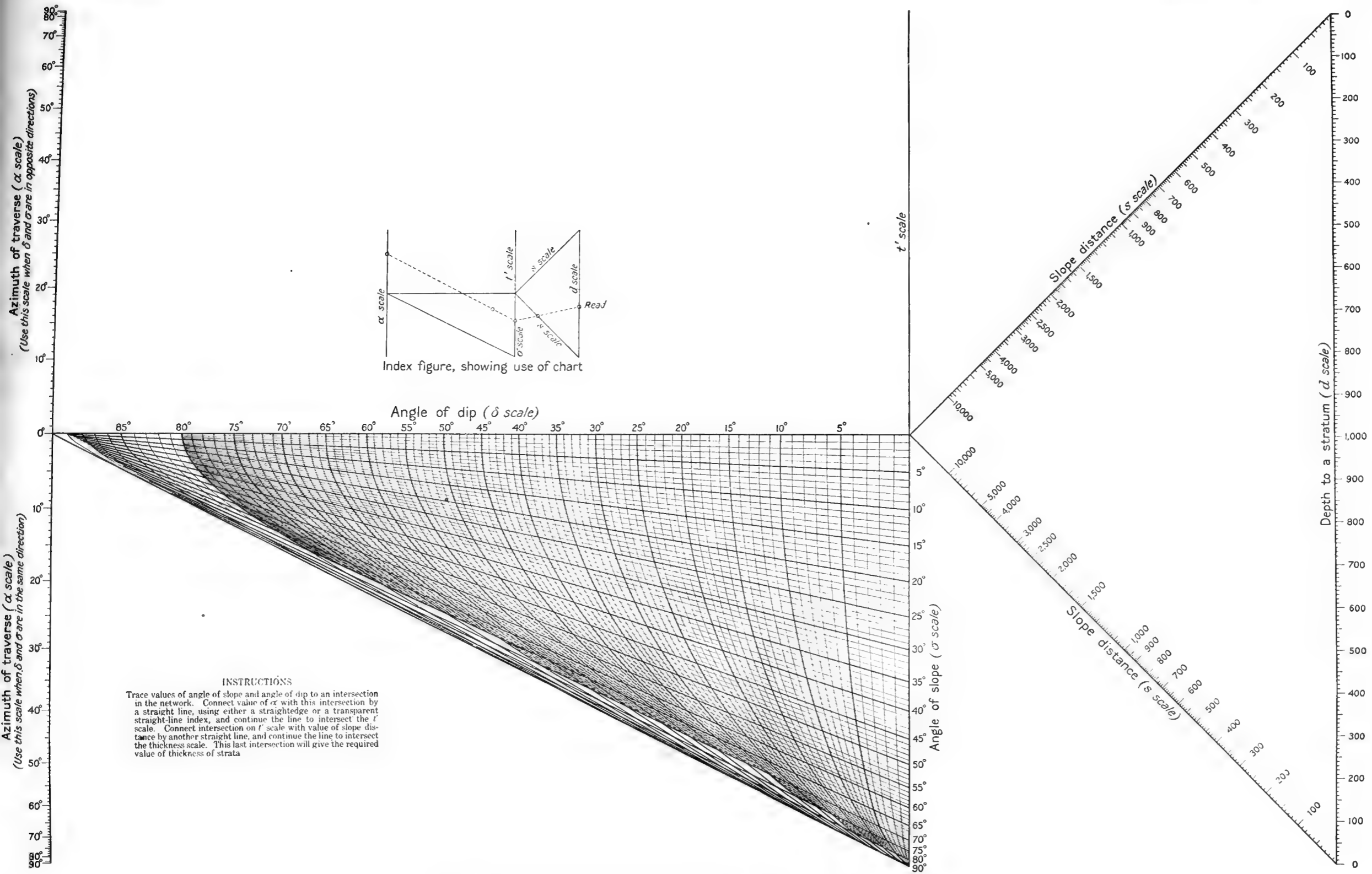
ALIGNMENT CHART FOR GRAPHIC COMPUTATION OF DEPTH TO A STRATUM.
