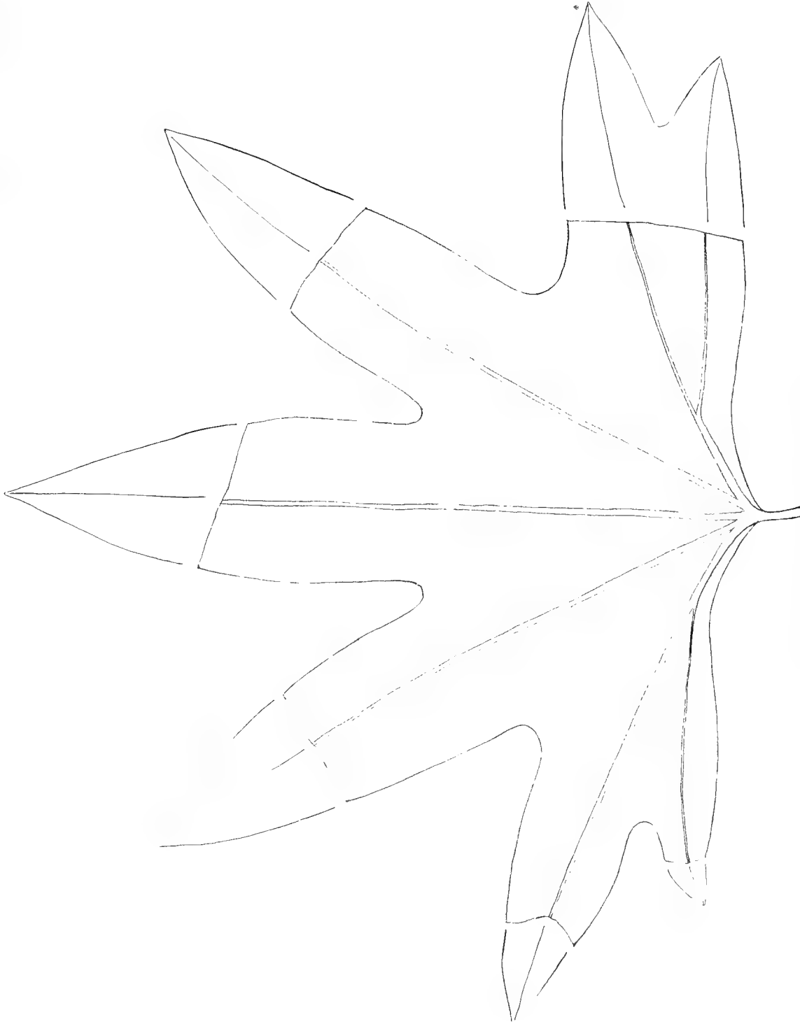
STERCULIA TOWNERI (LESQUEREUX) BERRY. From Cheyenne sandstone near Belvidere, Kans. About four-fifths natural size.
