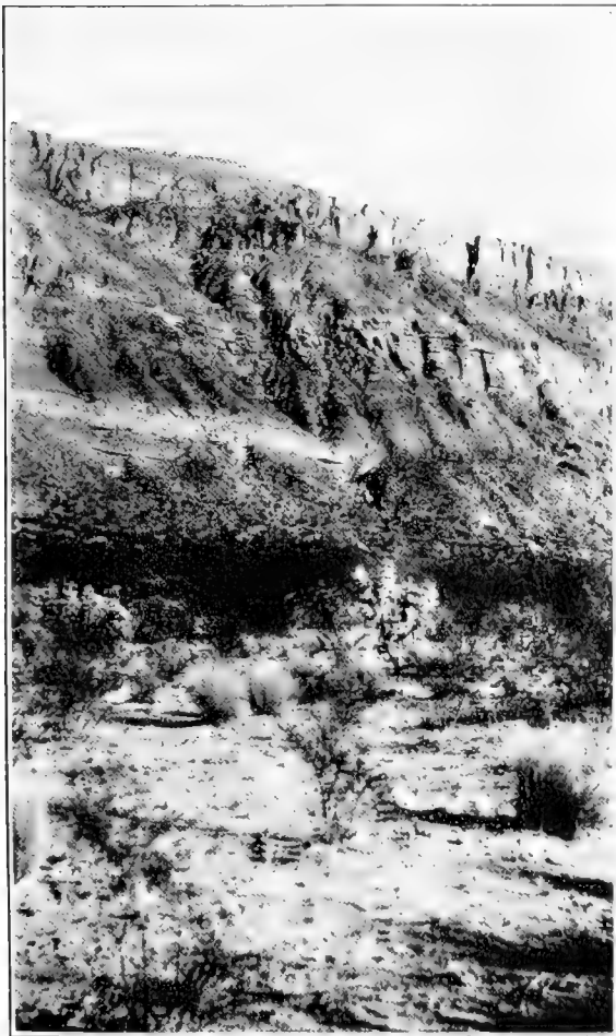
B. CLOSER VIEW OF MIDDLE PART OF SCARP SHOWN IN 1.
