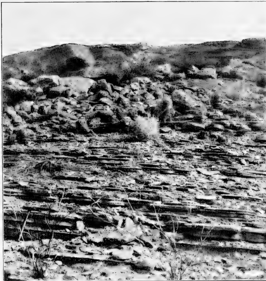
A. OSBORNE WASH, ABOUT 2 MILES SOUTHWEST OF OSBORNE'S WELL, YUMA COUNTY, ARIZ. A typical exposure of Tertiary limestone overlain by basalt.
