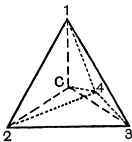
FIG. 12. Asymmetric carbon atom
