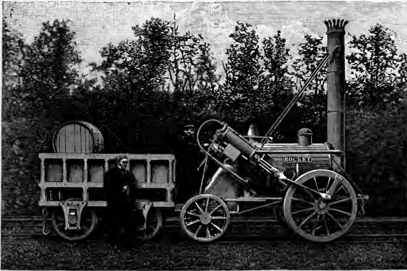
THE "ROCKET," 1829.
