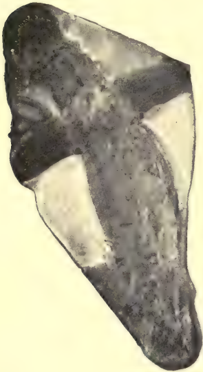
Nat. Hist. Mus. FOSSIL OF THE CLADOSELACHE, A DEVONIAN SHARK
