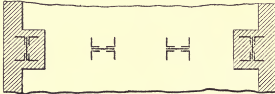
FIG. 11. CROSS-SECTION OF COLUMNS IN TRANSVERSE BENT
