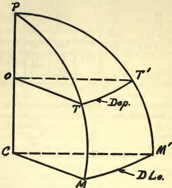
FIG. 19.—Parallel Sailing.
