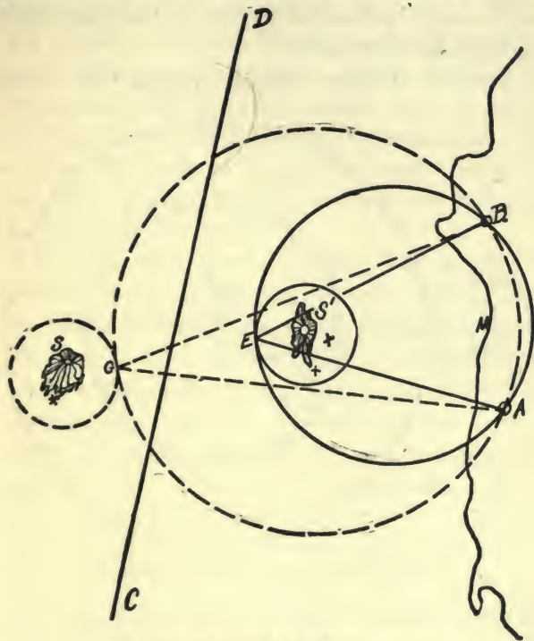
FIG. 13.—Horizontal Danger Angle.
