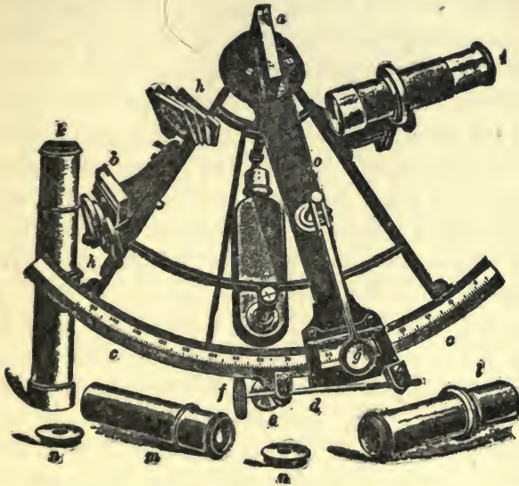
FIG. 6.—Sextant.
