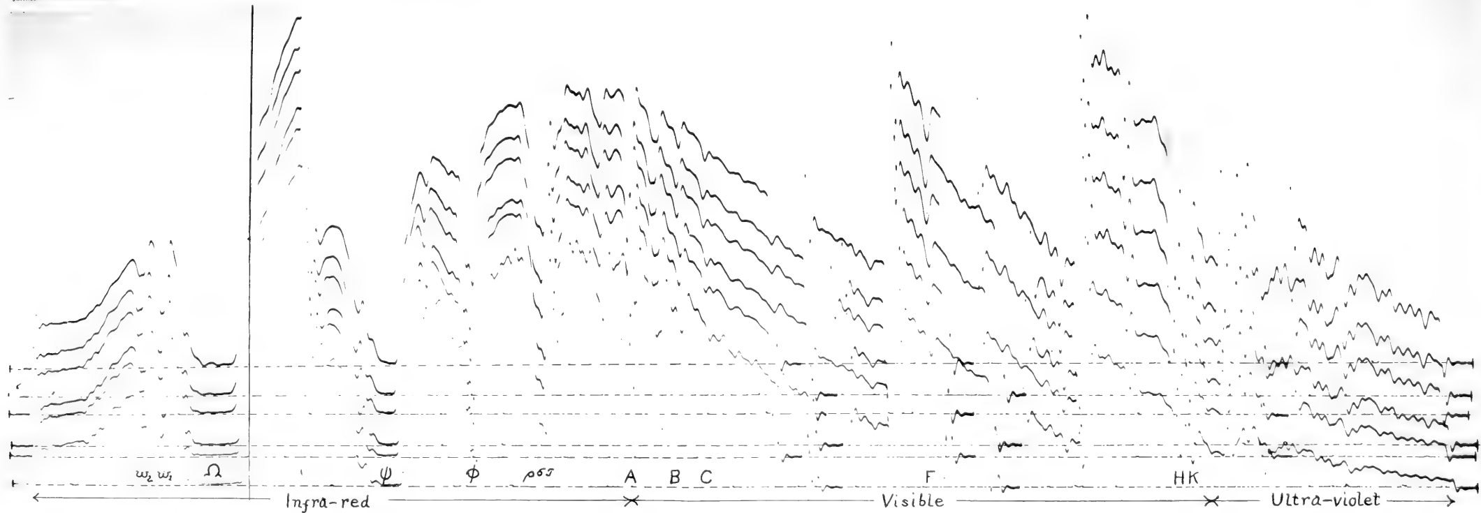
Biographs of the Solar Energy Spectrum, Observed at Monticima, Chile, March 18, 1925. Precipitable water, 1.4 centimeters.
