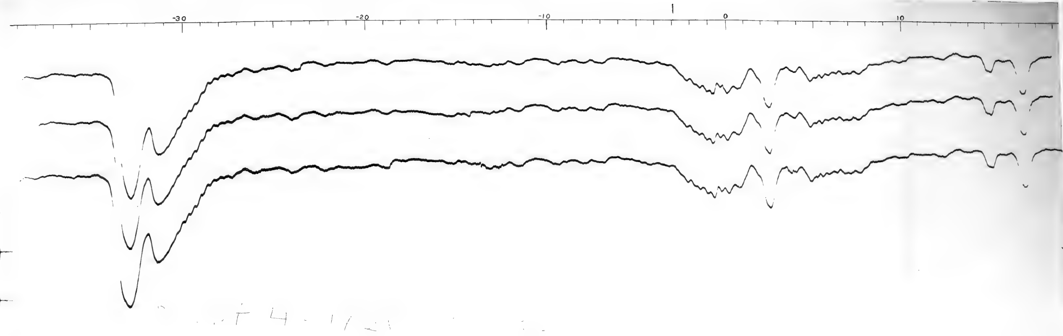
FRAGMENTS OF THE ISOSCELE PRISMATIC SOLAR SPECTRUM The A-region. Wavelengths 7600 to 8900 Angstroms
