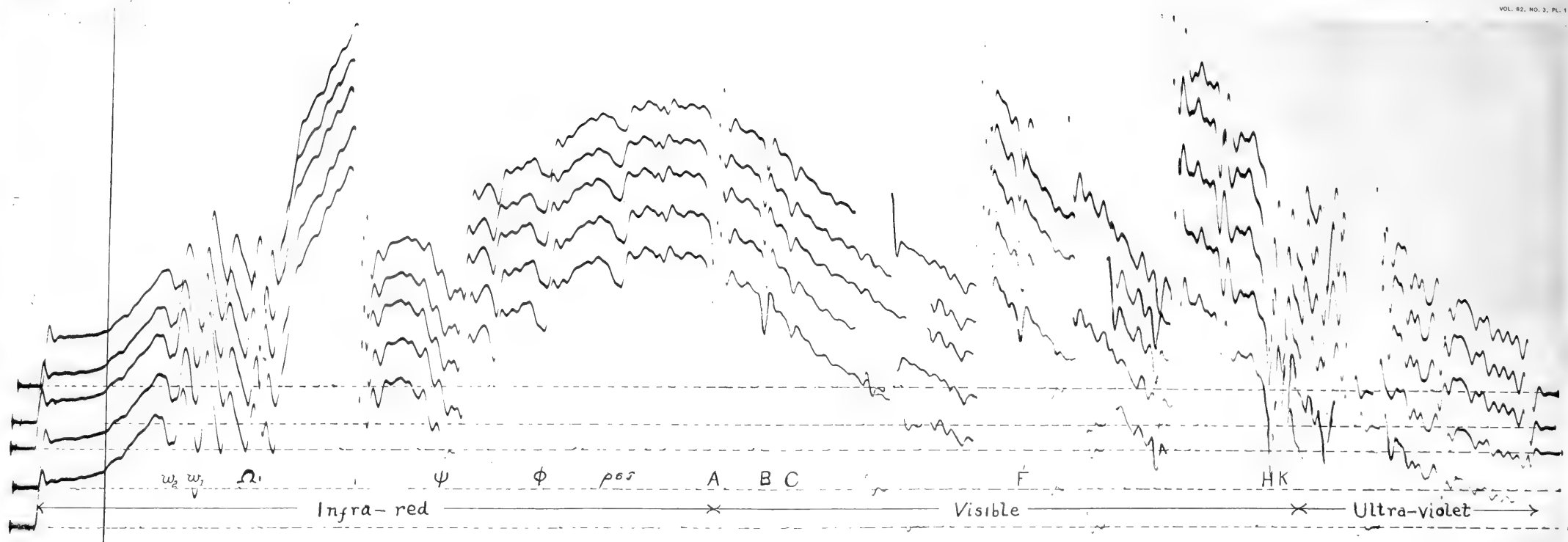
Biograph of the Sea of Energy Spectrum. Observed at Montezuma, Chile July 7, 1924. Precipitable water = 64 centimeters.
