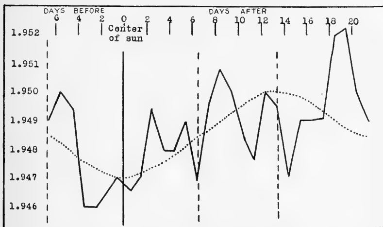
FIG. 1.—Calcium flocculi and solar radiation. The mean values of solar radiation received at the earth in calories per square centimeter per minute on days before and days after the passage of calcium flocculi across the central meridian of the sun. 1918-1920. Flocculi of 400 or more on the Ebro scale of values.
