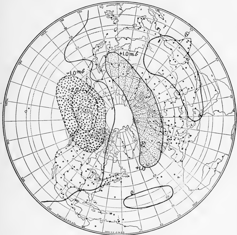
FIG. 8.—Longitude differences between high and low solar activity.
