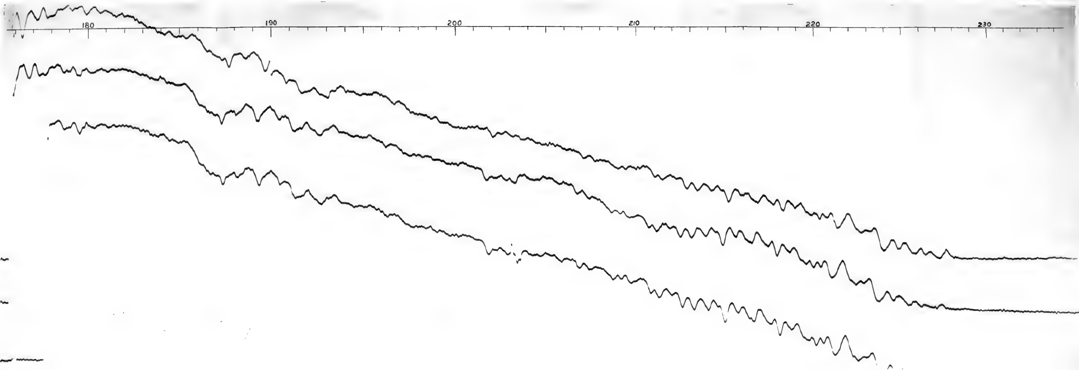
PHOTOGAMS OF THE INFRA-RED PRISMATIC SOLAR SPECTRUM The \eta region—Wave-lengths 1700 to 18200 Angstroms
