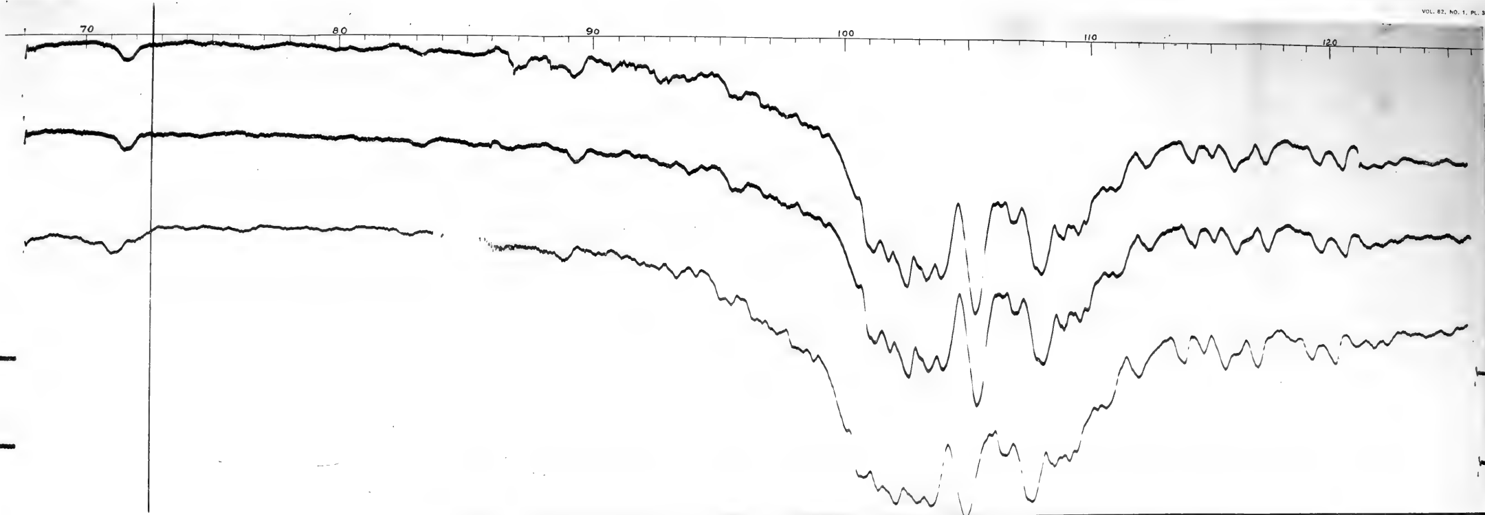
Fig. 1. — RECORD OF TIDE GAUGE WITH SEISM. SURF. AT ALBUQUERQUE, N.M., JULY 18, 1900. (12.00 A.M. EST.)
