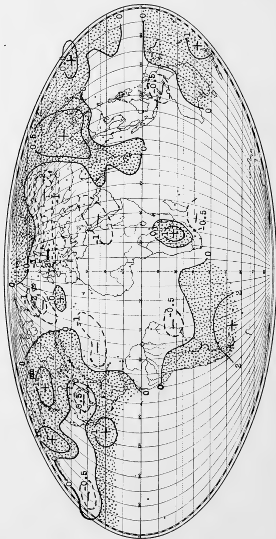
FIG. 25.—Differences between mean pressures with departures of solar radiation + .006 to + .010 and - .006 to - .010 . June to August.
