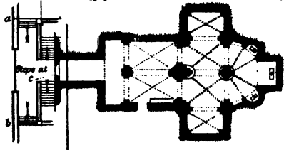
Plan of Chapel under Western Porch.
