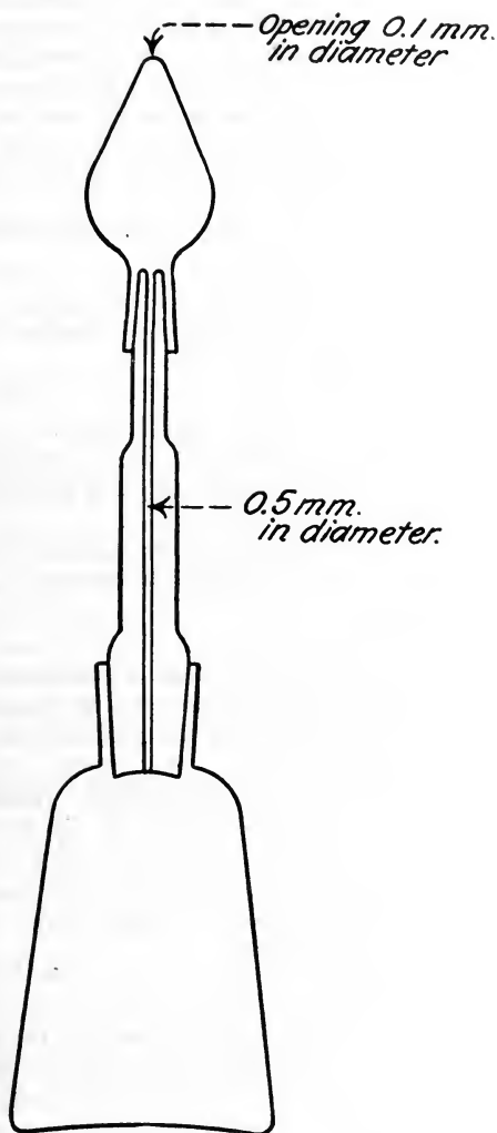
FIG. 1.—Pyknometer for very fluid liquids (actual size).
