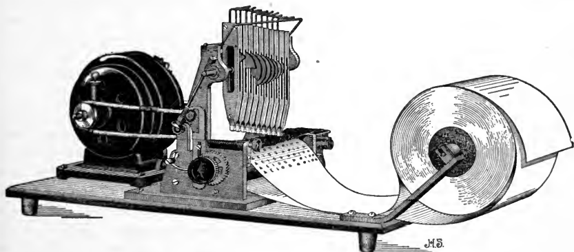
FIG. 3.—Machine for testing the life of typewriter ribbons.
