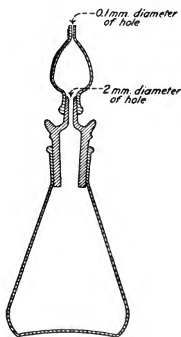
FIG. 2.—Pyknometer for viscous liquids (one-half actual size).
