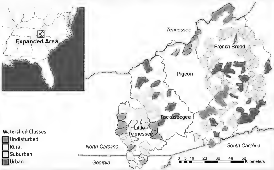
FIGURE 6.2 Watershed classification.
