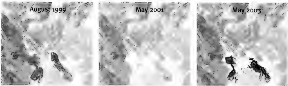
FIGURE 6.4 True colour Landsat 7 ETM+ images of Hamoun Lake, bordering Iran and Afghanistan. Source: http://earthobservatory.nasa.gov/Newsroom/NasaNews/2004/2004082717537.html
