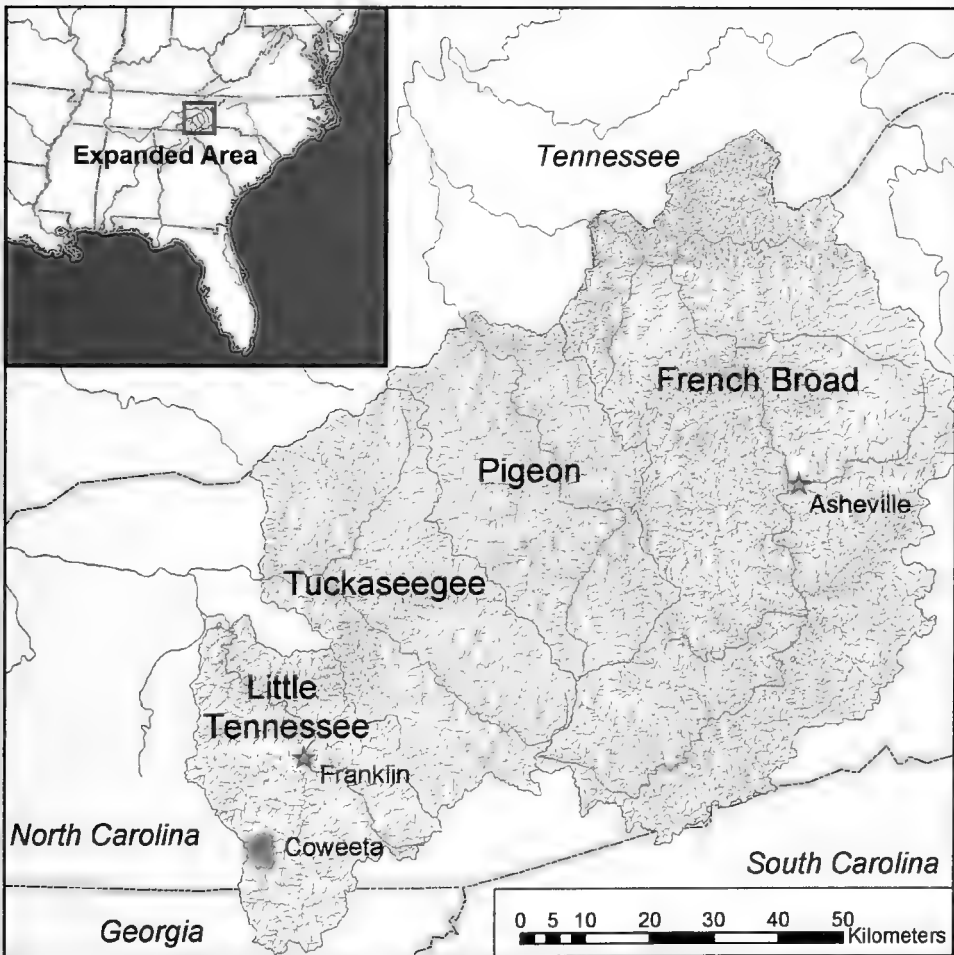
FIGURE 6.1 Study area, including four watersheds, in western North Carolina.
