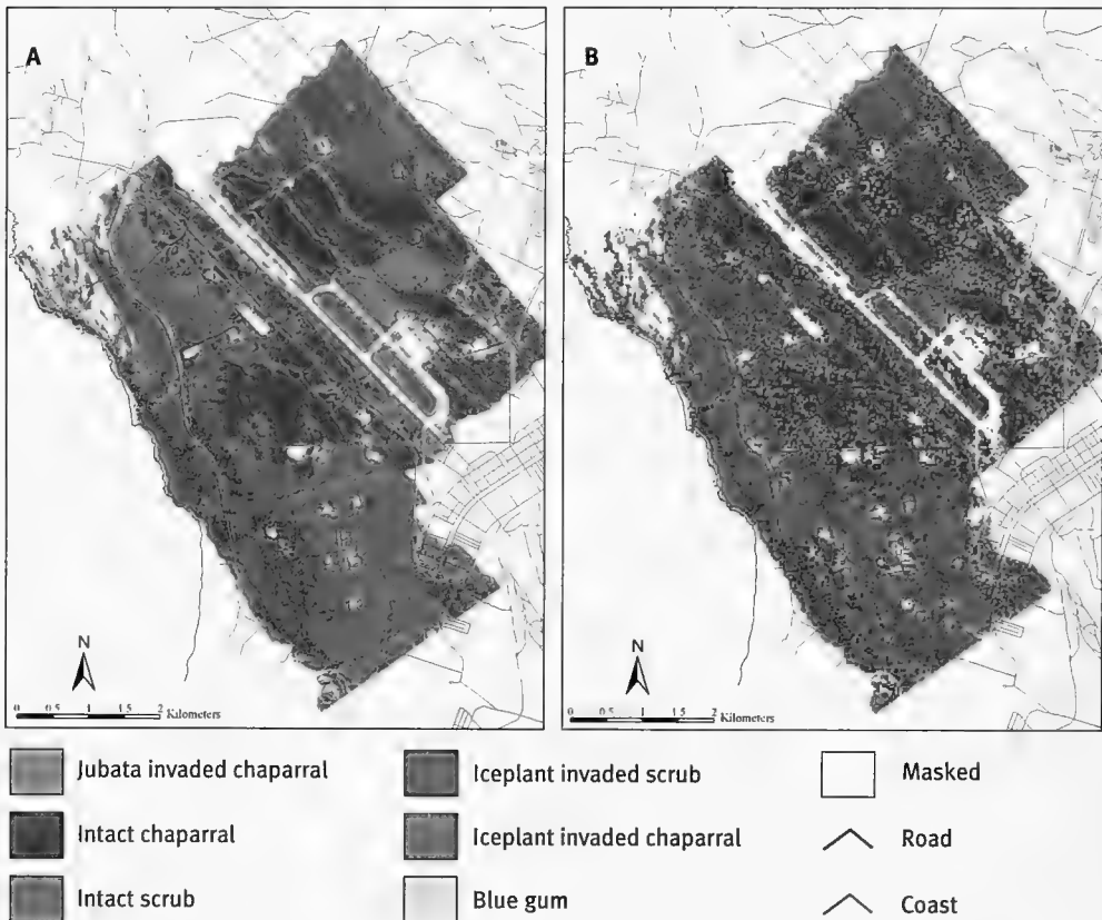
FIGURE 11.7 Classification of six vegetation types at Vandenberg Air Force Base, California, USA: A. Hyperspectral (AVIRIS) image (4 m and 174 wavebands) and B. Landsat ETM (30 m and 6 wavebands) 3 .
