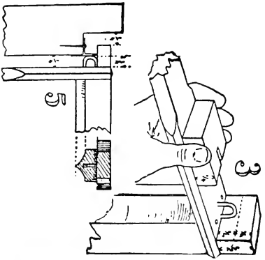
Method of fastening Comb-foundation.
