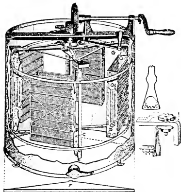
Four-frame Extractor with Automatic Reversing Gear.
