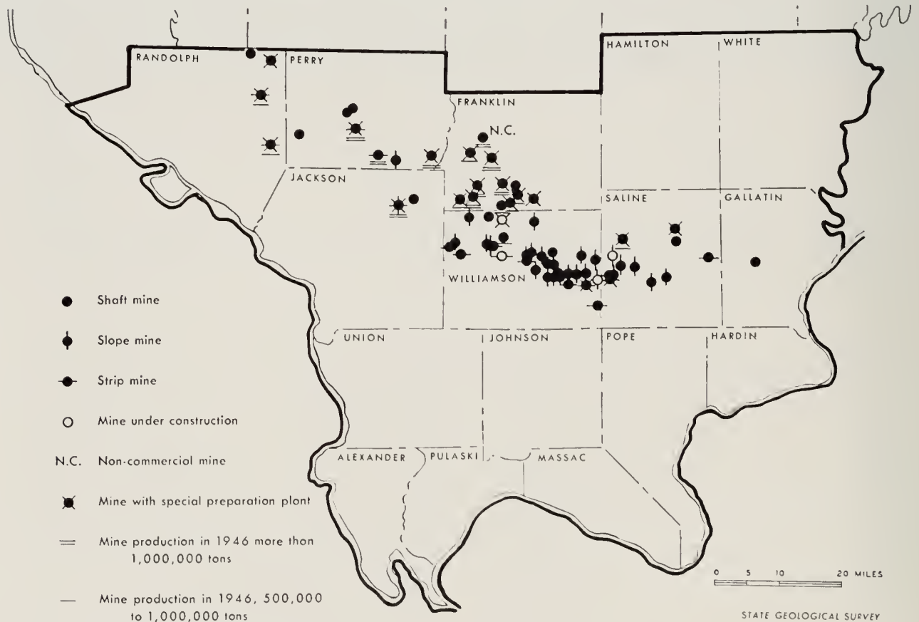
Fig. 28. Map of shipping mines in Southern Illinois, 1947. (G. H. Cady, Coal Division, State Geological Survey.)
