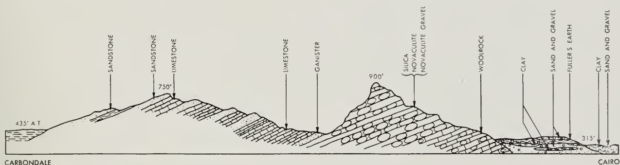
Fig. 45. Cross section of Southern Illinois showing geological formations exposed and their relation to mineral resources. The vertical scale of the drawing is greatly exaggerated. For map of mineral resources, see Fig. 46. (J. E. Lamar, Industrial Minerals Division, State Geological Survey.)
