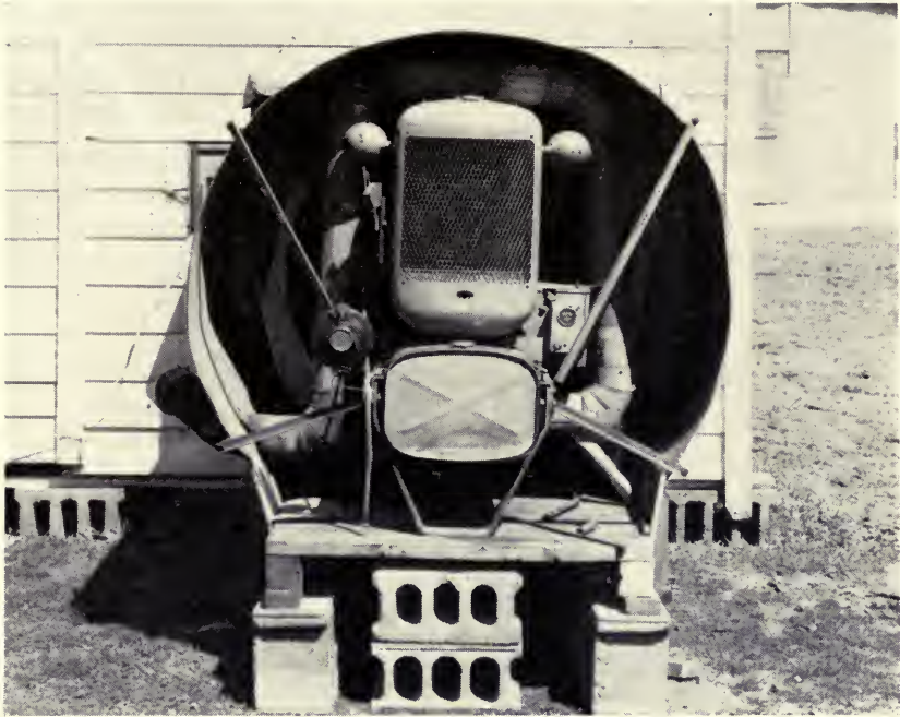
This portable drying unit consisted of a propeller-type fan connected to the drive shaft of a stationary engine. The shield directed inlet air past the engine so as to utilize the waste heat for drying. (See Tests 3 and 4, Table 6.) (Fig. 15)
