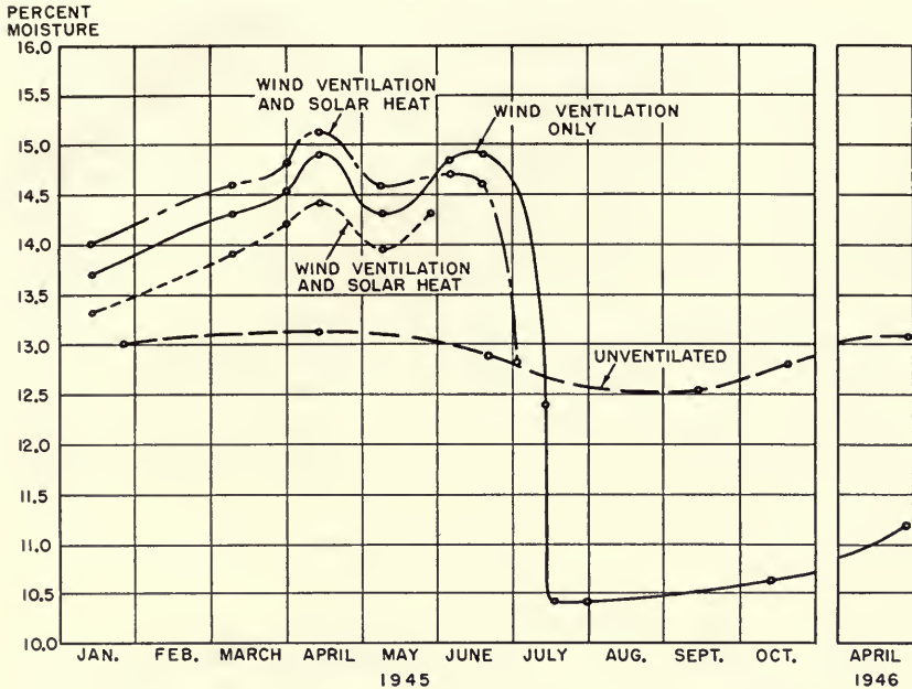
In three bins ventilated as illustrated in Fig. 10, wind ventilation did not reduce moisture during winter and spring but rather tended to increase it. Moistures did not change in the unventilated check bin. (Fig. 11)
