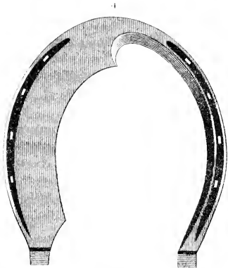
Side weight shoe for hind foot.
