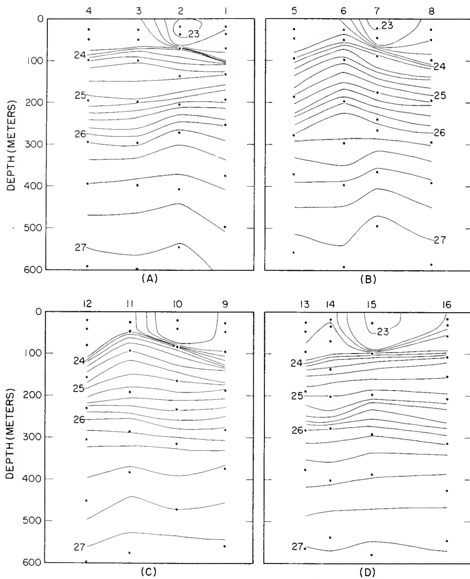
Fig. 6.--H. M. Smith cruise 1. Profiles of sigma-t, isopleth interval 0.2. A. Stations 1-4, B. Stations 5-8, C. Stations 9-12, and D. Stations 13-16.
