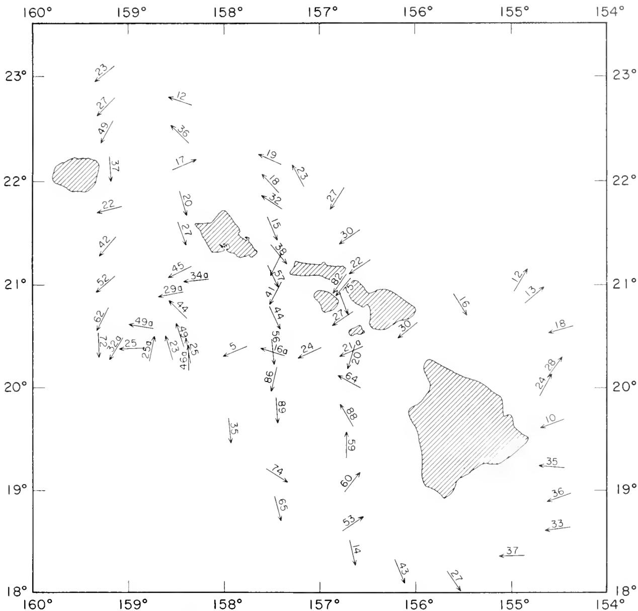
Fig. 25. --H. M. Smith cruise 12. Current vectors computed from GEK measurements, velocities in \text{cm/sec} . "a" indicates observations made during the recheck of the area south of Oahu at the end of the cruise.
