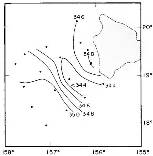
Fig. 9.--H. M. Smith cruise 1. Surface salinity in ‰, isohaline interval 0.2 ‰.
