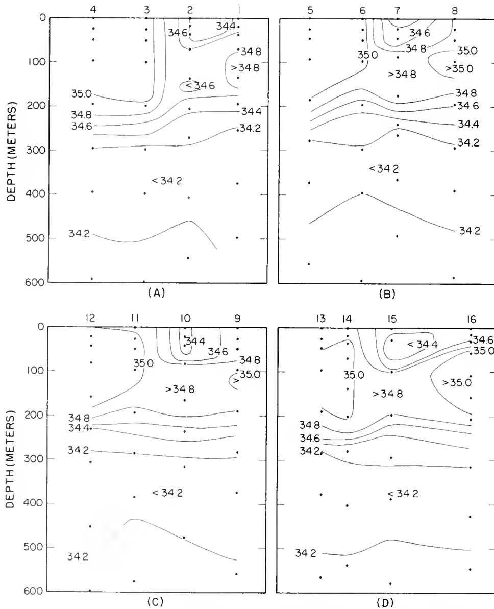
Fig. 8.-- H. M. Smith cruise 1. Profiles of salinity in ‰, isohaline interval 0.2 \text{ ‰} . A. Stations 1-4, B. Stations 5-8, C. Stations 9-12, and D. Stations 13-16.
