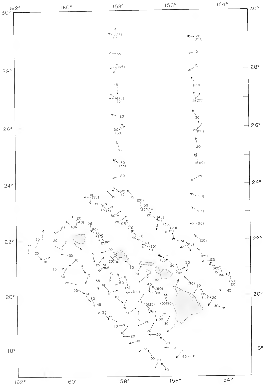
Figure 16.--Geomagnetic electrokinetograph (GEK) current speeds in cm./sec. and directions, H. M. Smith cruise 20, March 1953. Dashed arrows and numbers in parentheses indicate observations with floated electrodes.
