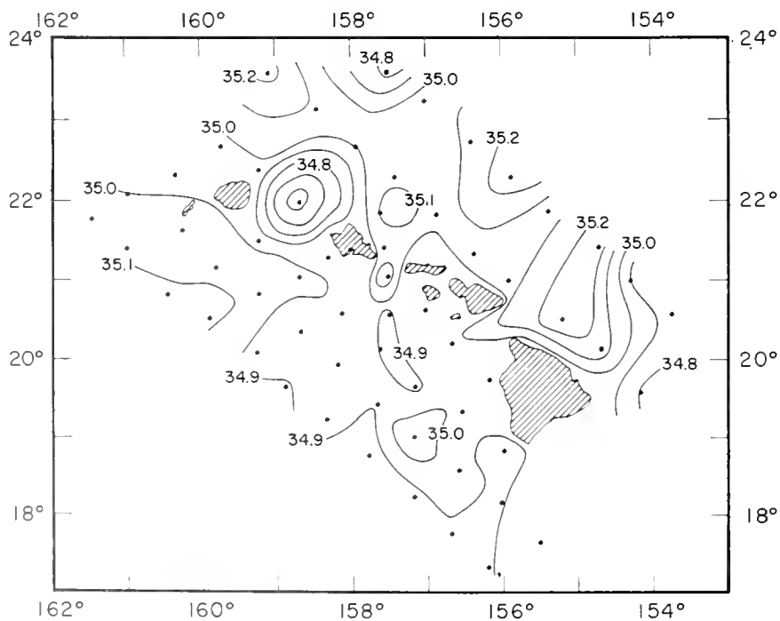
Figure 27. --Surface salinity in ^{\circ}/\text{oo} , H. M. Smith cruise 21, August 1953. Contour interval 0.1^{\circ}/\text{oo} .
