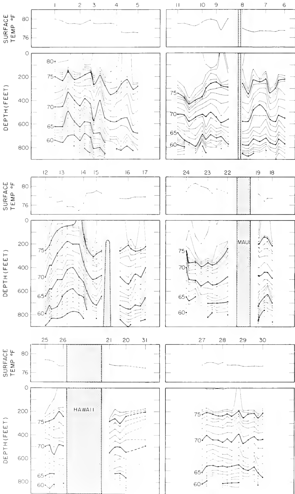
Figure 10. -- Vertical bathythermograph temperature ( ^{\circ} F.) sections from stations 5 to 1, 6 to 11, 17 to 12, 18 to 24, 31 to 25, and 30 to 27, H. M. Smith cruise 17, September 1952. The upper panels show the surface bucket temperatures in ^{\circ} F.
