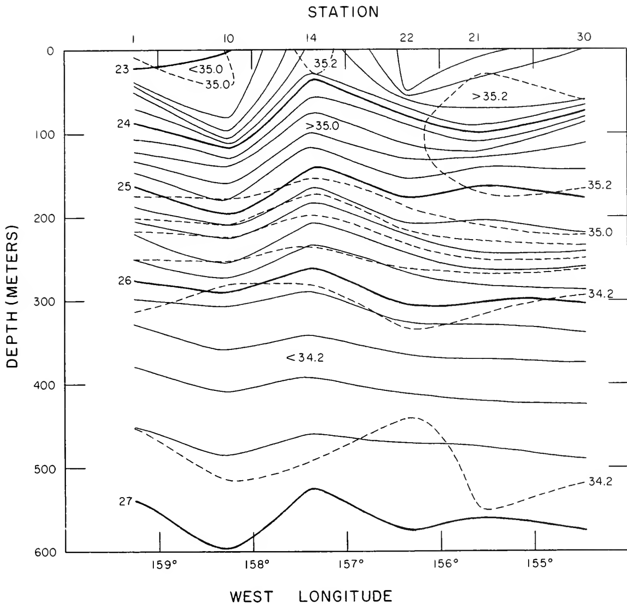
Figure 6.--Density ( \sigma\text{-t} ) section (solid lines) and salinity ( ^{\circ}/\text{oo} ) section (dashed lines) through stations 1, 10, 14, 22, 21, and 30, H. M. Smith cruise 17, September 1952. Sigma-t contour interval is 0.2, salinity contour interval 0.2 ^{\circ}/\text{oo} .
