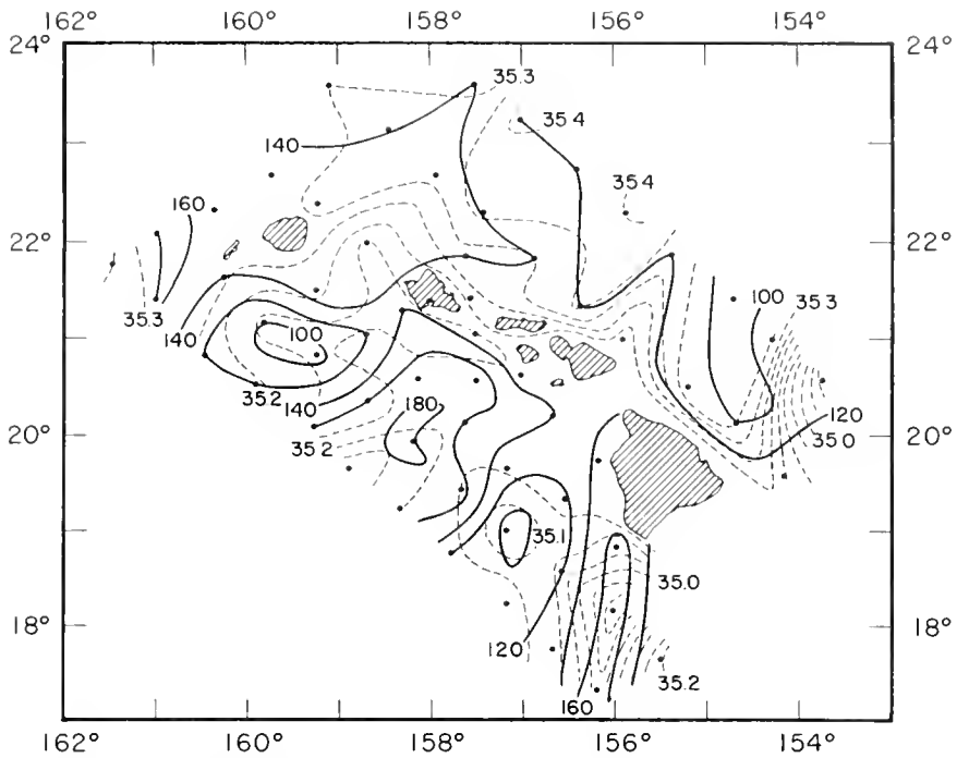
Figure 31. -- Bathymetric chart (depth in meters) of the 24.5 sigma-t surface, H. M. Smith cruise 21, August 1953. Contour interval 20 m. Dashed lines indicate the salinity ( ^{\circ}/\text{oo} ) distribution on the surface with contour intervals of 0.05^{\circ}/\text{oo} .
