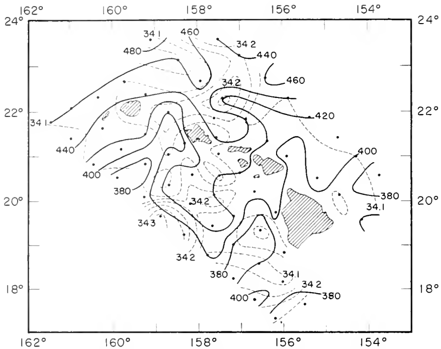
Figure 33. --Bathymetric chart (depth in meters) of the 26.5 sigma-t surface, H. M. Smith cruise 21, August 1953. Contour interval 20 m. Dashed lines indicate the salinity ( ^{\circ}/\text{oo} ) distribution on the surface with contour intervals of 0.05^{\circ}/\text{oo} .
