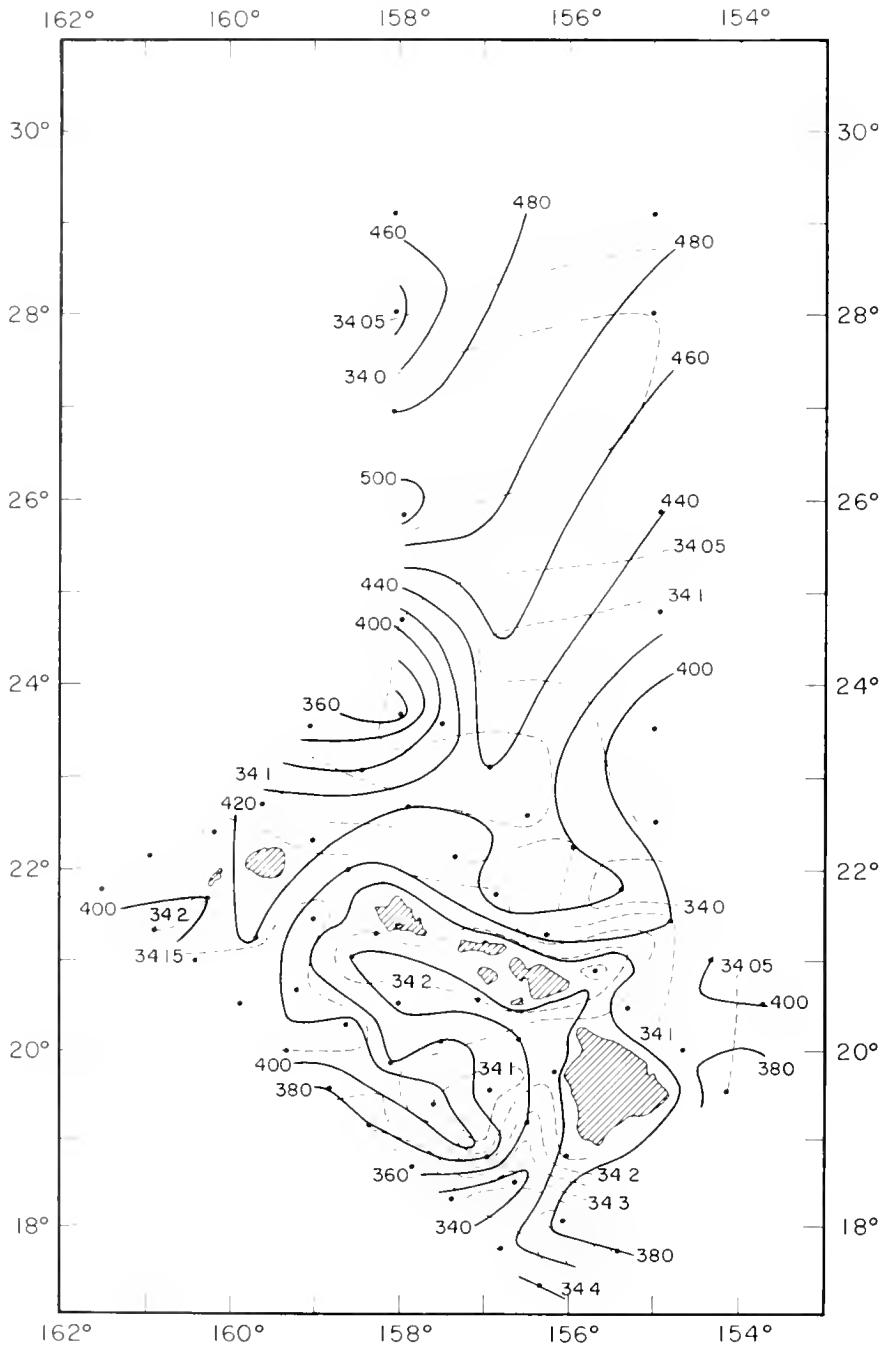
Figure 18. --Bathymetric chart (depth in meters) of the 26.5 sigma-t surface, H. M. Smith cruise 20, March 1953. Contour interval 20 m. Dashed lines indicate the salinity (‰) distribution on the surface with contour intervals of 0.05 ‰.
