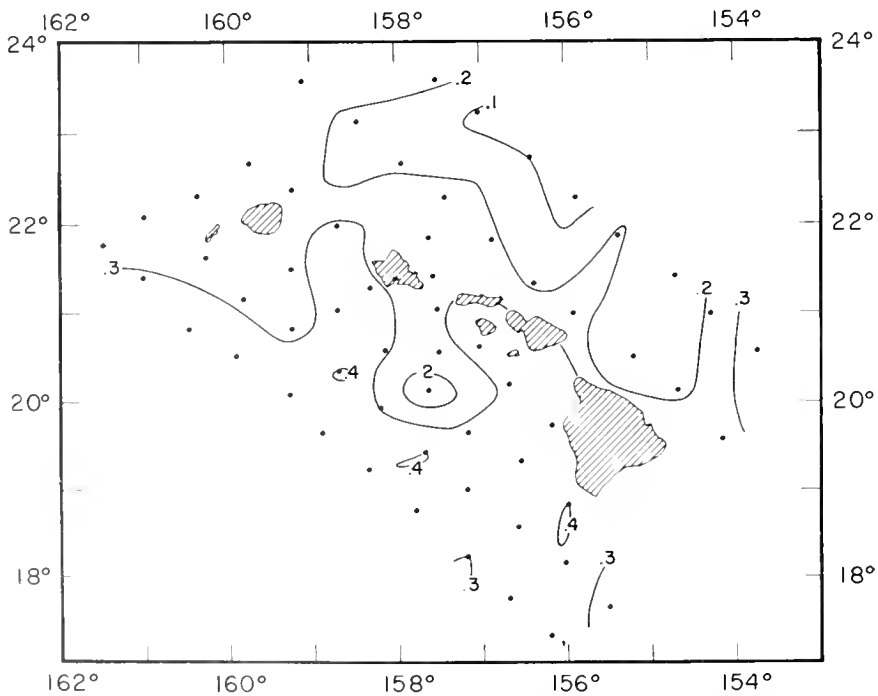
Figure 37. --Phosphate-phosphorus distribution ( \mu\text{g-at/l} ) on the 24.5 \sigma\text{-t} surface, H. M. Smith cruise 21, August 1953. Contour interval 0.1 \mu\text{g-at/l} .
