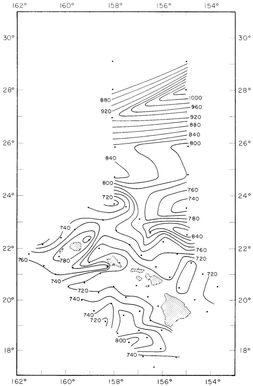
Figure 19.--Bathymetric chart (depth in meters) of the 27.2 sigma-t surface, H. M. Smith cruise 20, March 1953. Contour interval 20 m.
