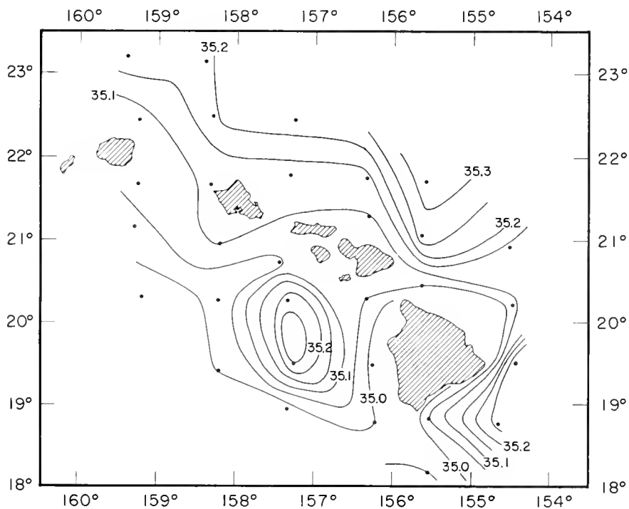
Figure 3.--Surface salinity in ^{\circ}/\text{oo} , H. M. Smith cruise 17, September 1952. Contour interval 0.05^{\circ}/\text{oo} .
