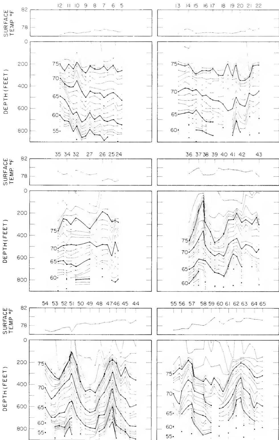
Figure 35. -- Vertical bathythermograph temperature ( ^{\circ}\text{F.} ) sections from stations 5 to 12, 22 to 13, 24 to 35, 43 to 36, 44 to 54, and 65 to 55, H. M. Smith cruise 21, August 1953. The upper panels show the surface bucket temperatures in ^{\circ}\text{F.}
