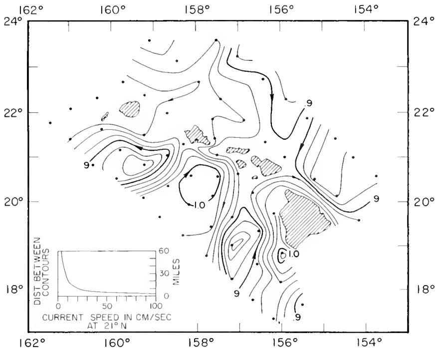
Figure 32. -- Dynamic height anomalies (dynamic meters) at the surface relative to 250 m., H. M. Smith cruise 21, August 1953. Contour interval 0.02 dynamic meters.
