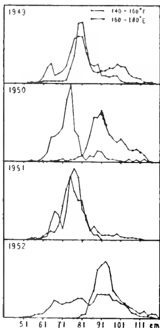
Figure 6. --Length frequency of albacore taken in the North Pacific, by years. The two curves represent different ranges of longitude, but the original figure is too small to distinguish them.
