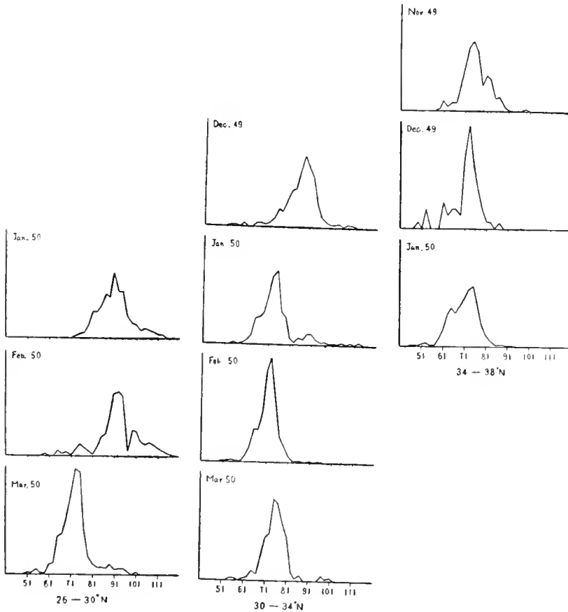
Figure 7.--Albacore length frequency by months in the North Pacific at 140^{\circ} - 150^{\circ} E., 1949-50.
