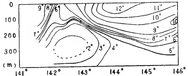
Figure 3. --Vertical temperature section off Kinkazan (from Hydrographic Office reports).
