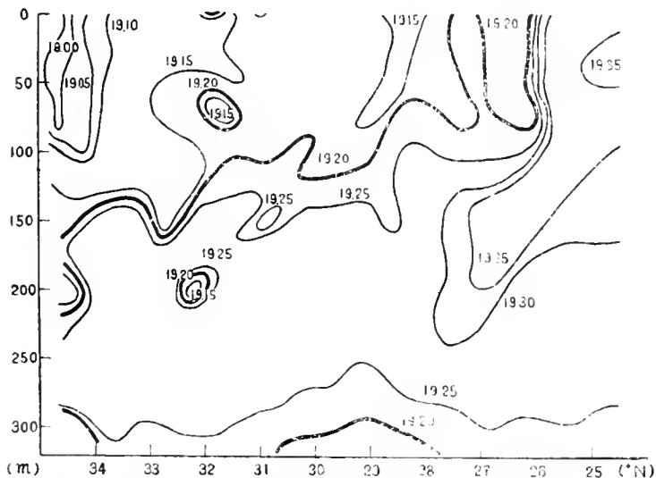
Figure 3b. --Chlorinities between Cape Nojima and Iwojima.
