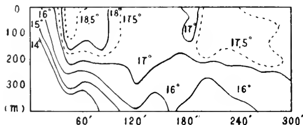
Figure 5. -- Vertical temperature section 300 miles southeast of Cape Nojima.
