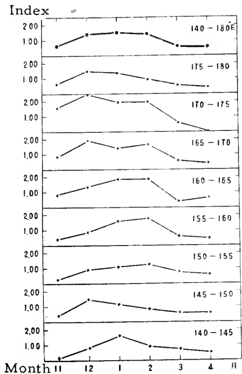
Figure 1.--Indices of seasonal changes in catch rates.
