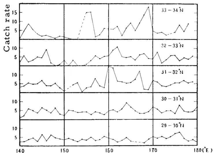
Figure 2.--Catch rates by latitude.
