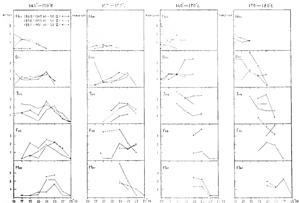
Figure 1. -- Catch rates by month and area.
