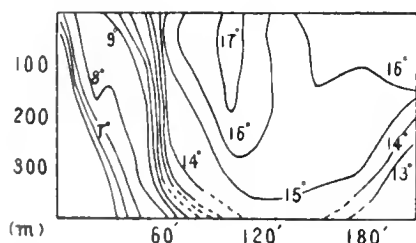
Figure 2. --Vertical temperature section due east of Cape Inubō (1936). From Semi-ann. Rpts. Oceanog. Observations.
