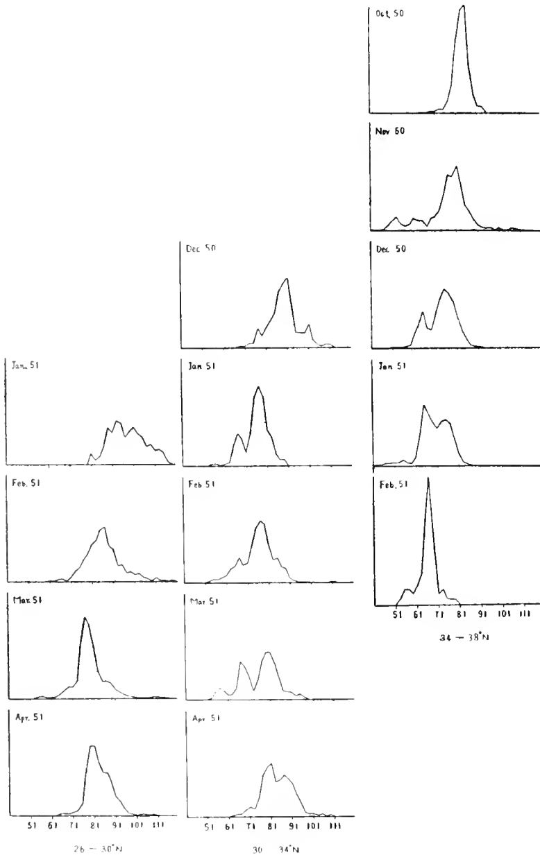
Figure 8.--Albacore length frequency by months in the North Pacific at 140°-150°E., 1950-51.
