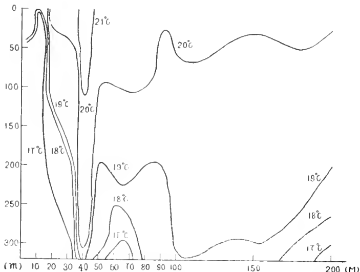
Figure 4a. --Water temperatures on a 200-mile section due east of Inubozaki, December 8-9, 1938.
