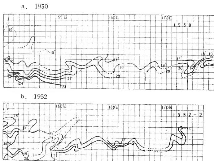
Figure 1. --Distribution of surface water temperatures in the North Pacific.
