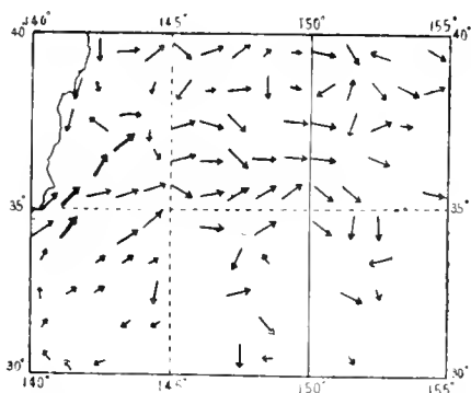
Figure 2. -- Vector current chart (based on J. H. O. 6031A)
