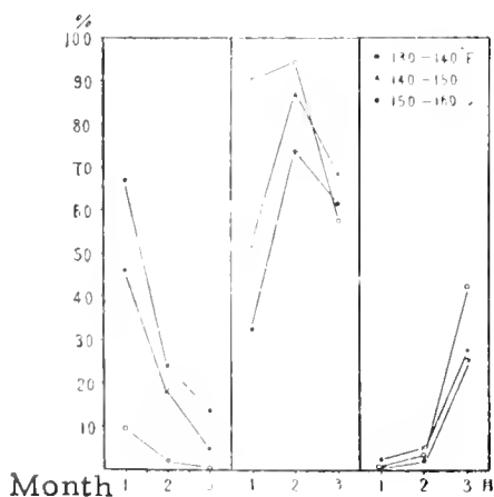
Figure 7.--Percentages of small, medium, and large albacore in the catch at 28°-30° N., 130°-160° E. Left panel - over 85 cm. Center panel - 65-85 cm. Right panel - below 65 cm.
