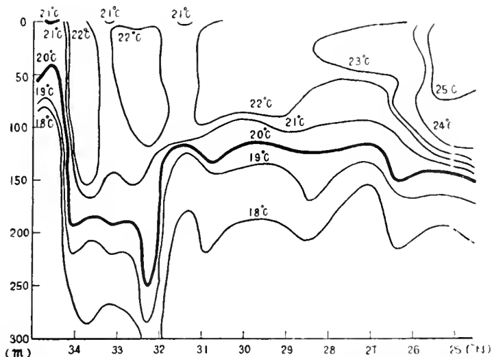
Figure 3a. --Water temperatures between Cape Nojima and Iwojima.
