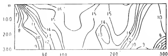
Figure 2. --Vertical temperature section 300 miles due east of Cape Inubō, 1936.
