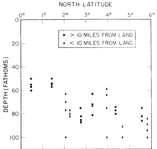
Figure 4. --Latitudinal variation in depth of the deepest hook on longline sets, as determined by sounding tubes, 157°48'W. - 161°57'W. longitude, John R. Manning cruise 27, October 1955.
