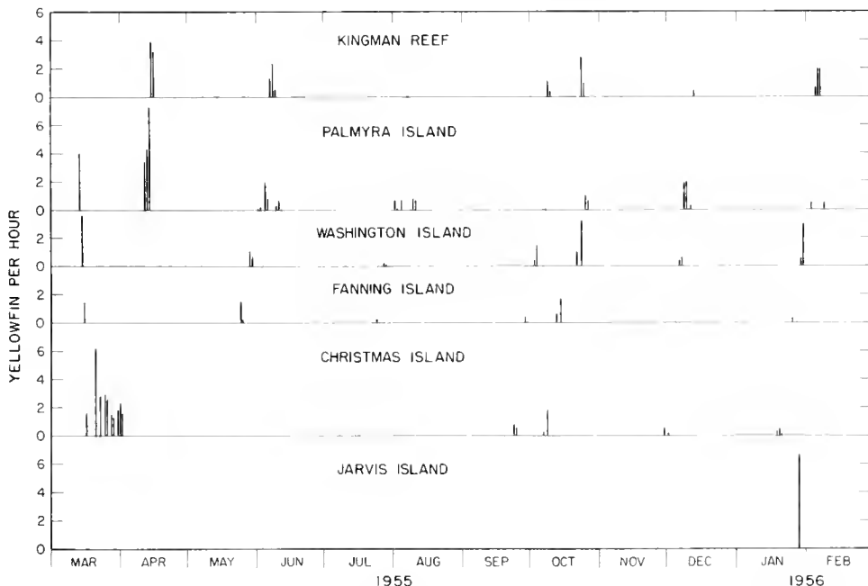
Figure 9.--Yellowfin troll catch rates in the Line Islands, March 1955 to February 1956.
