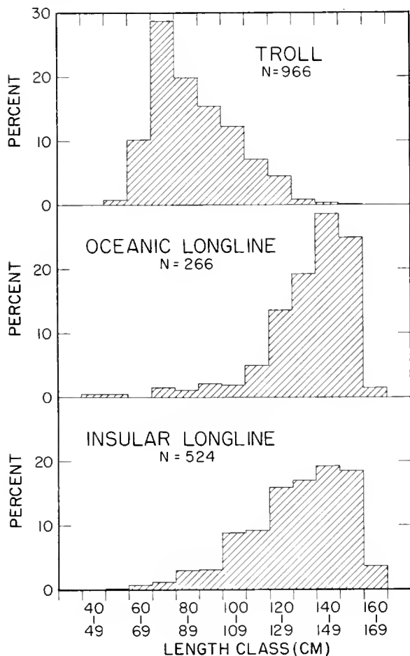
Figure 7.--Length frequency distributions of oceanic and insular yellowfin caught by longlining and trolling (data in Appendix, table 5).
