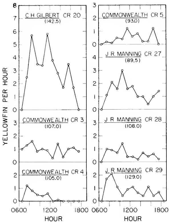
Figure 8.--Yellowfin troll catch rates in the Line Islands arranged by time of day (data in Appendix, table 6). The figures in the parentheses are the total number of hours trolled.
