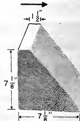
Figure 2. --Sectional cut of the Dalles-type weir crest. Arrow indicates direction of flow.
